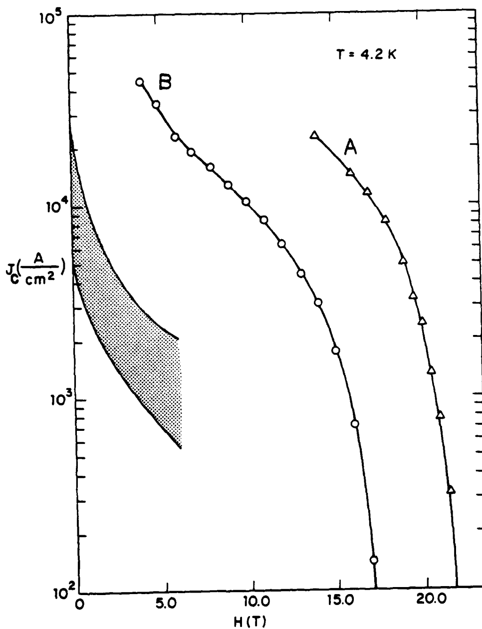
Figure 2.4 J_c vs. H for the two Cu-V 3 Ga samples. Sample B has roughly the amount of Ga required to form stoichiometric V 3 Ga, sample A about twice as much as is necessary. The shaded area encompasses the data of Chen and Tsuei (1976).
