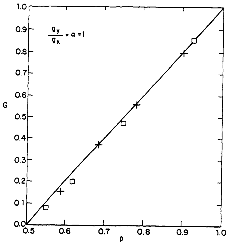
Figure 5.5 Conductance vs. concentration for \alpha=1 from the EMT (solid curve), numerical simulation (+) and the RG ( \square ).
