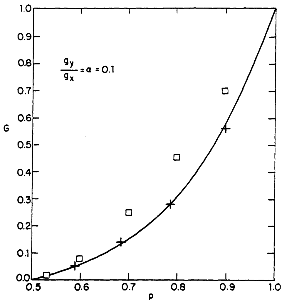
Figure 5.7 Conductance vs. concentration for \alpha=0.1 from the EMT (solid curve), numerical simulation (+) and the RG (Q).
