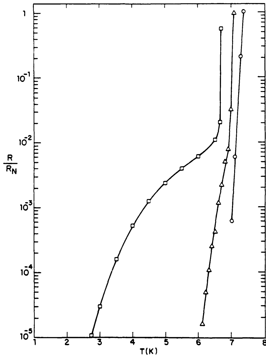
Figure 4.3 Semilogarithmic plot of resistance against temperature for sample A. The current ranges from 182mA to 10μA from left to right.
