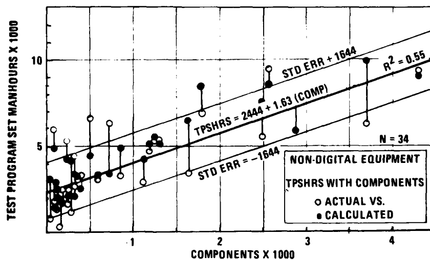
Figure 12. - Comparison of calculated and actual TPSHRS with components
