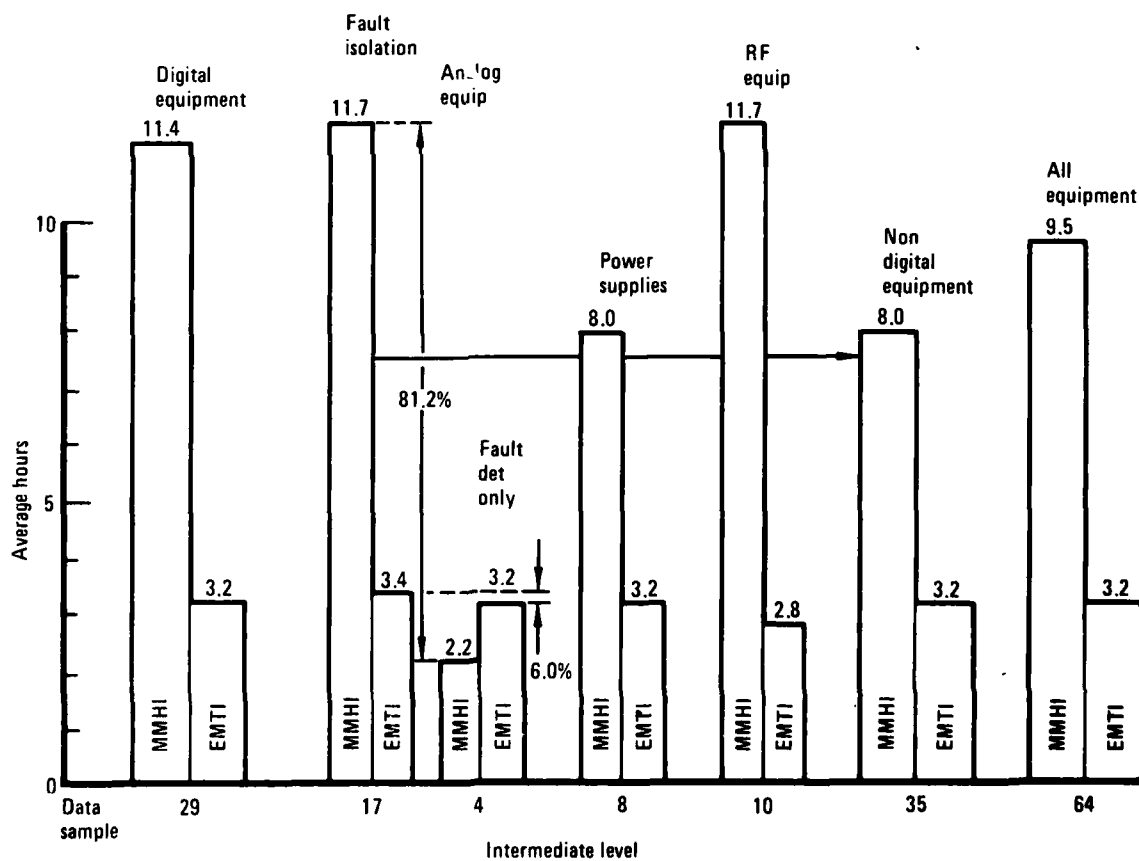
Figure 13. - S-3A Maintenance time averages.
