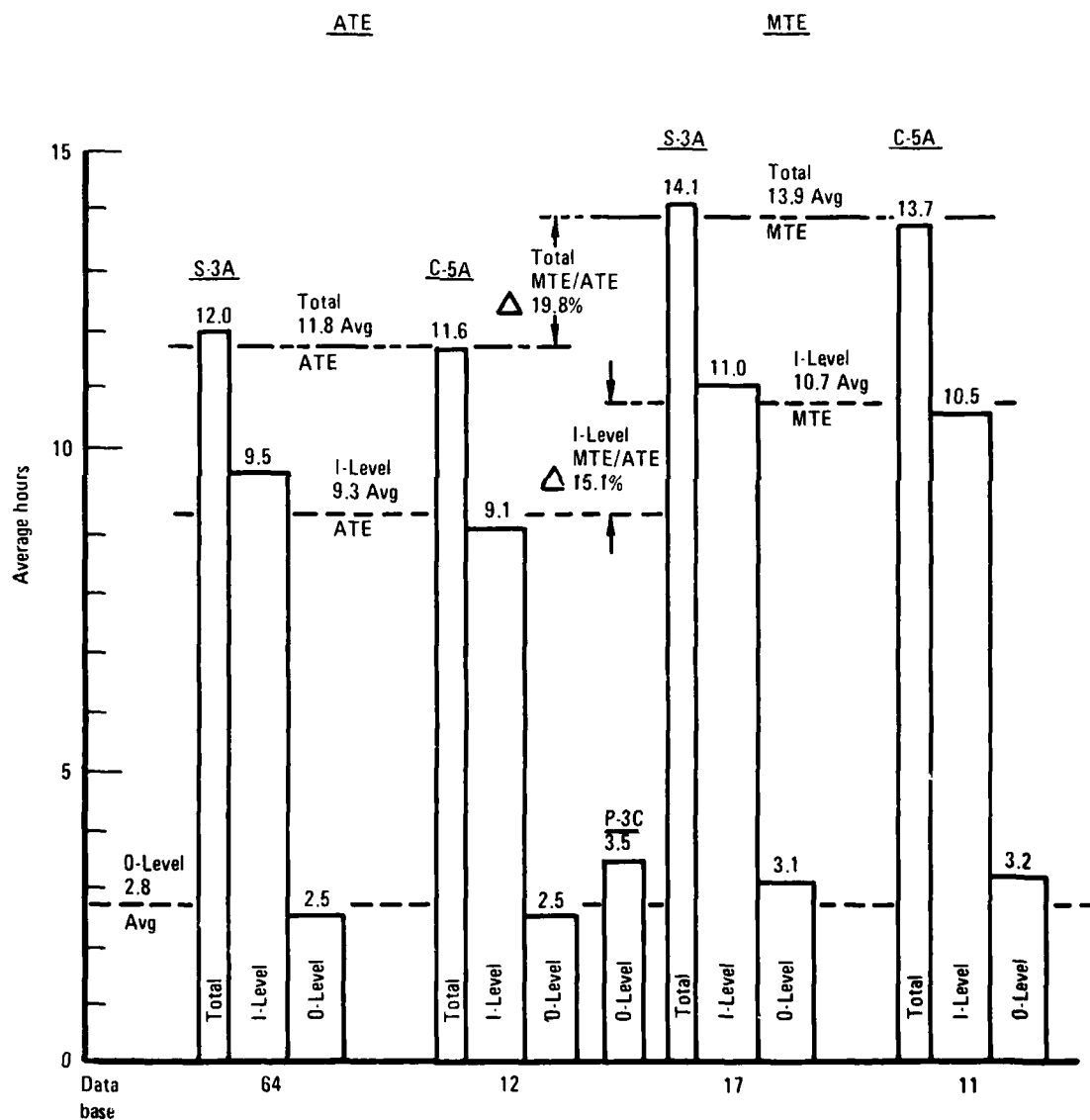
Figure 14. - Comparison of ATE and MTE S-3A and C-5A airborne equipment maintenance manhours.
