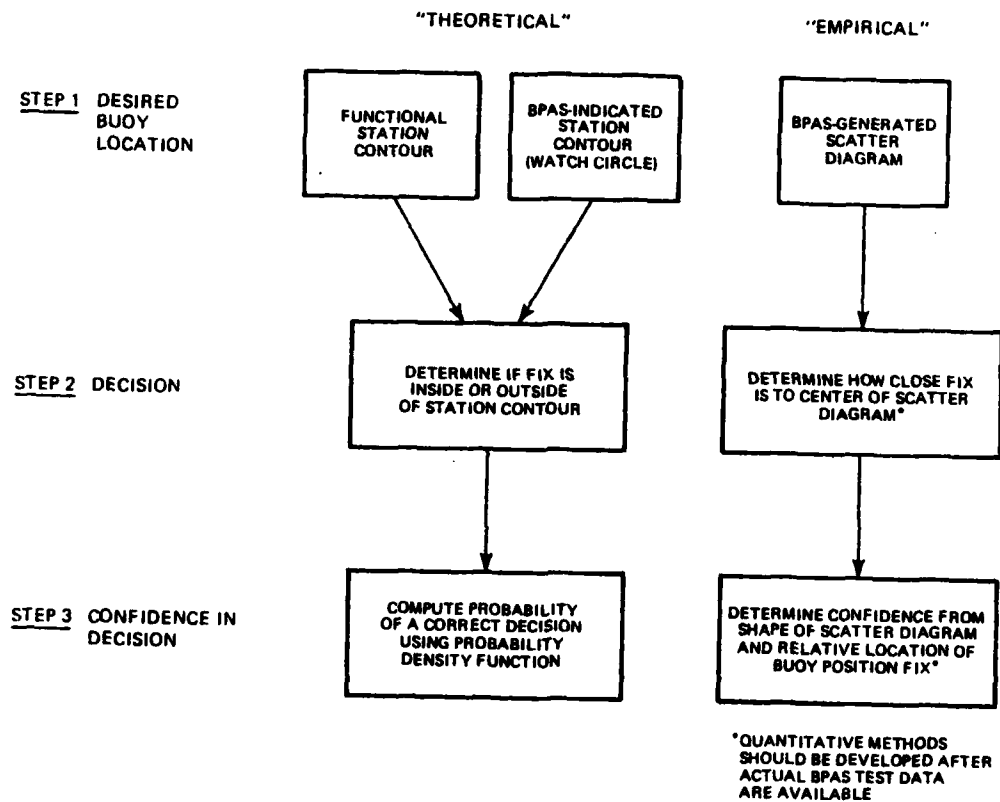
Figure 4.4-3 Summary of Candidate BPAS Decision Algorithms
