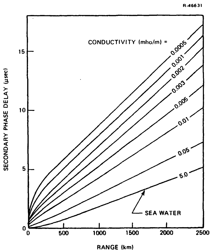
Figure A.5-3 Secondary Phase Delay for a Homogeneous Propagation Path
