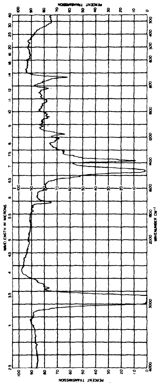
Figure 3. IR spectrogram of 30W oil.
