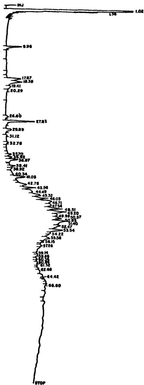
Figure 13. GLC chromatogram of 90W oil reference material.
