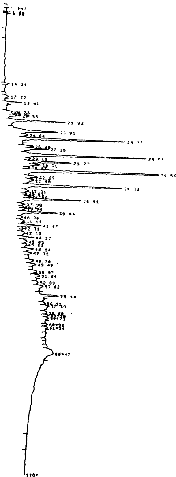
Figure 24. Chromatogram of field sample.
