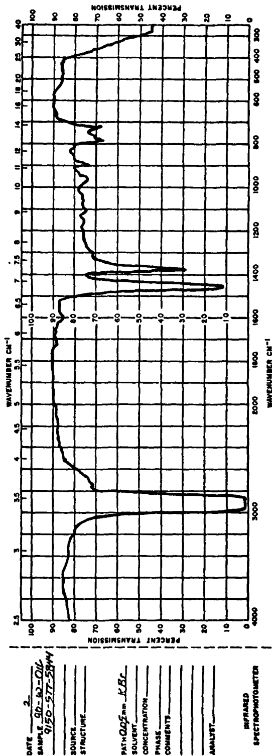
Figure 4. IR spectrogram of 90W oil.
