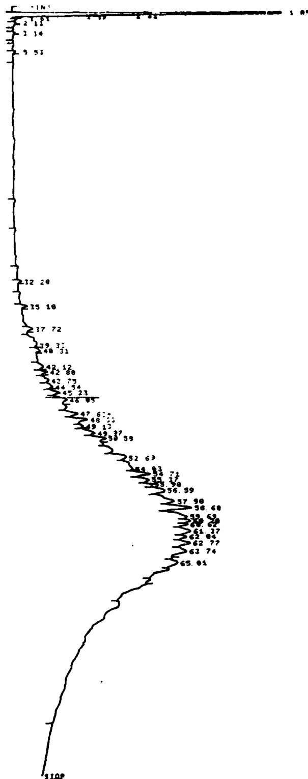
Figure 12. GLC chromatogram of 30W oil reference material (Fort Lewis).
