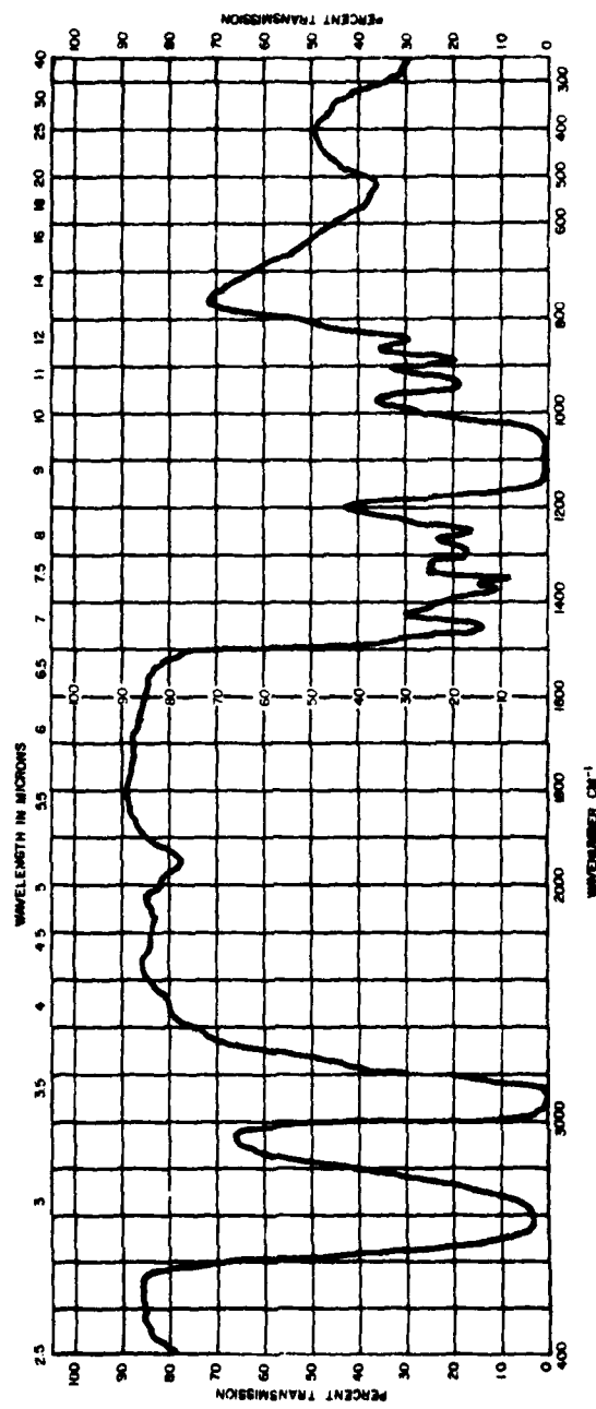
Figure 7. IR spectrum of brake fluid.
