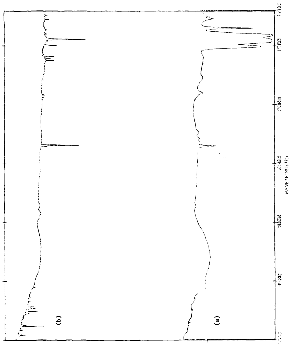
Fig. 3.4 FT-IR spectra of \text{NF}_3 , \text{BF}_3 and \text{F}_2 mixtures.
