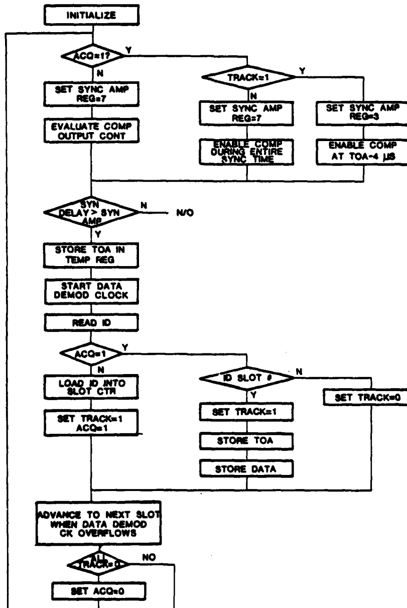
FIG. B-2 SYNC PROCESSING FLOW CHART
