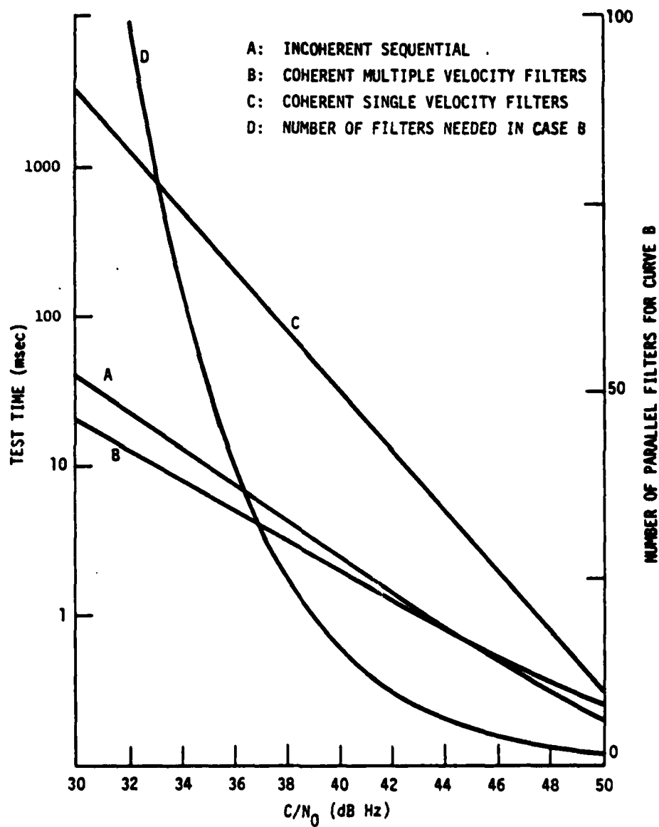
FIG. A-1 TEST TIME ON ONE CODE PHASE FOR INITIAL CODE ACQUISITION FOR MAXIMUM FREQUENCY UNCERTAINTY OF \pm 4 kHz
