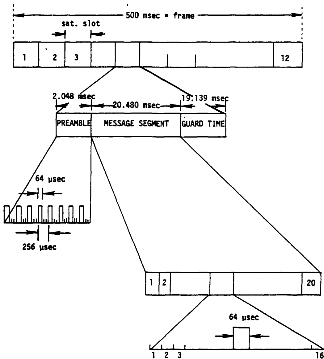
FIG. 4-1 PULSED SIGNAL FORMAT
