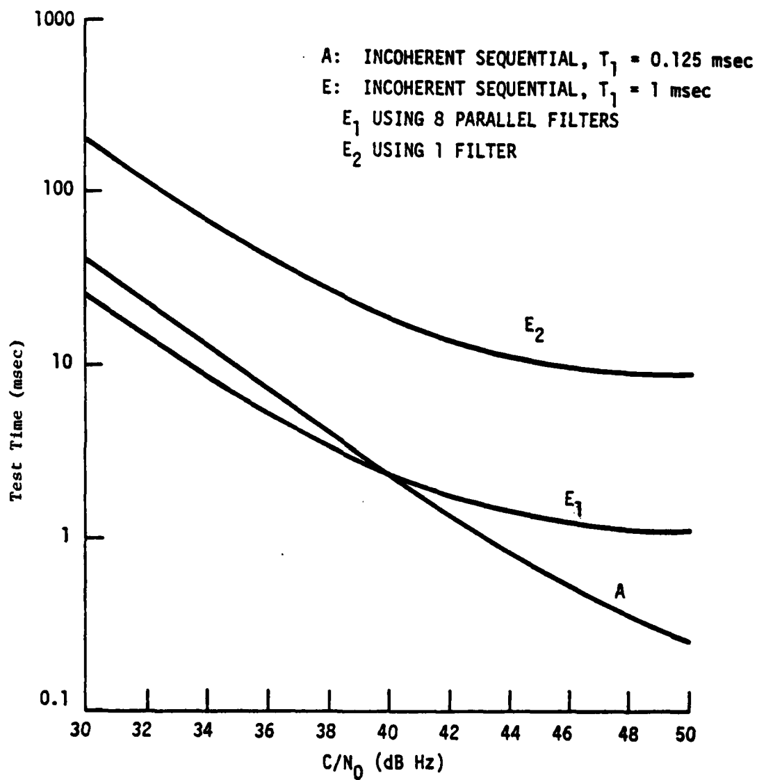
FIG. A-2 TEST TIME ON ONE CODE PHASE FOR INITIAL CODE ACQUISITION FOR MAXIMUM FREQUENCY UNCERTAINTY
