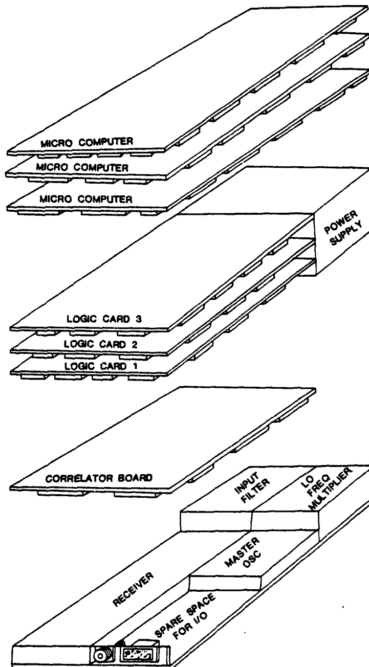
FIG. 4-6 PACKAGING OF TDMA PULSED GPS RECEIVER
