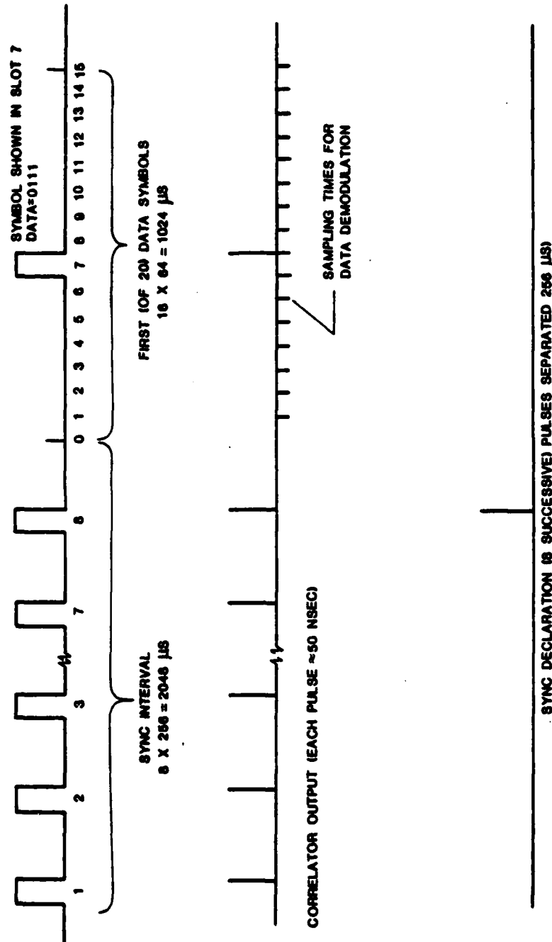
FIG. B-1 PROCESSING WAVEFORMS
