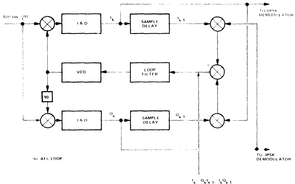
Figure B-2. Phase and frequency tracking loops
