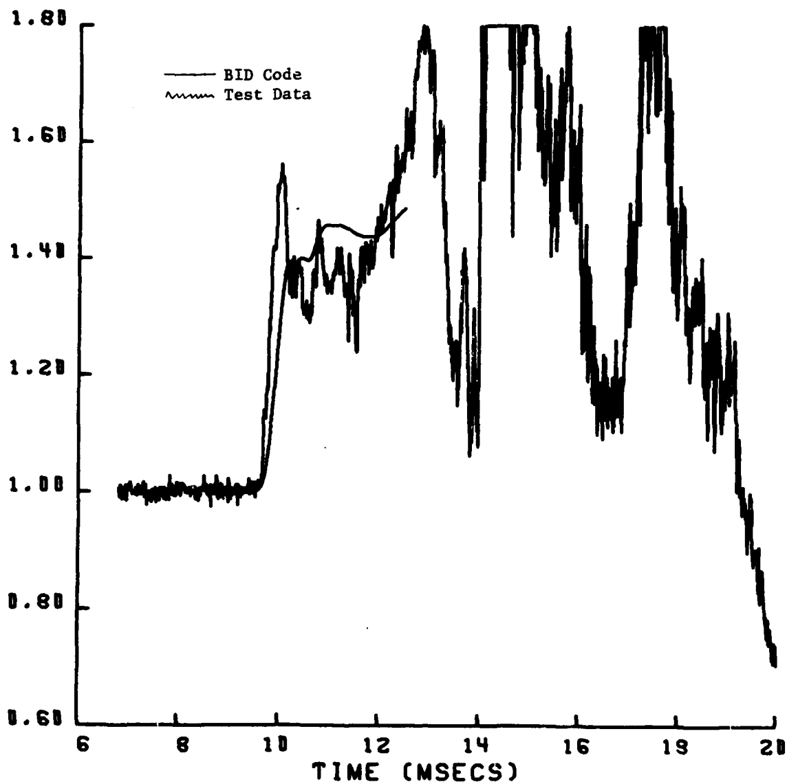
Figure 5.14g. Transducer 1832.
