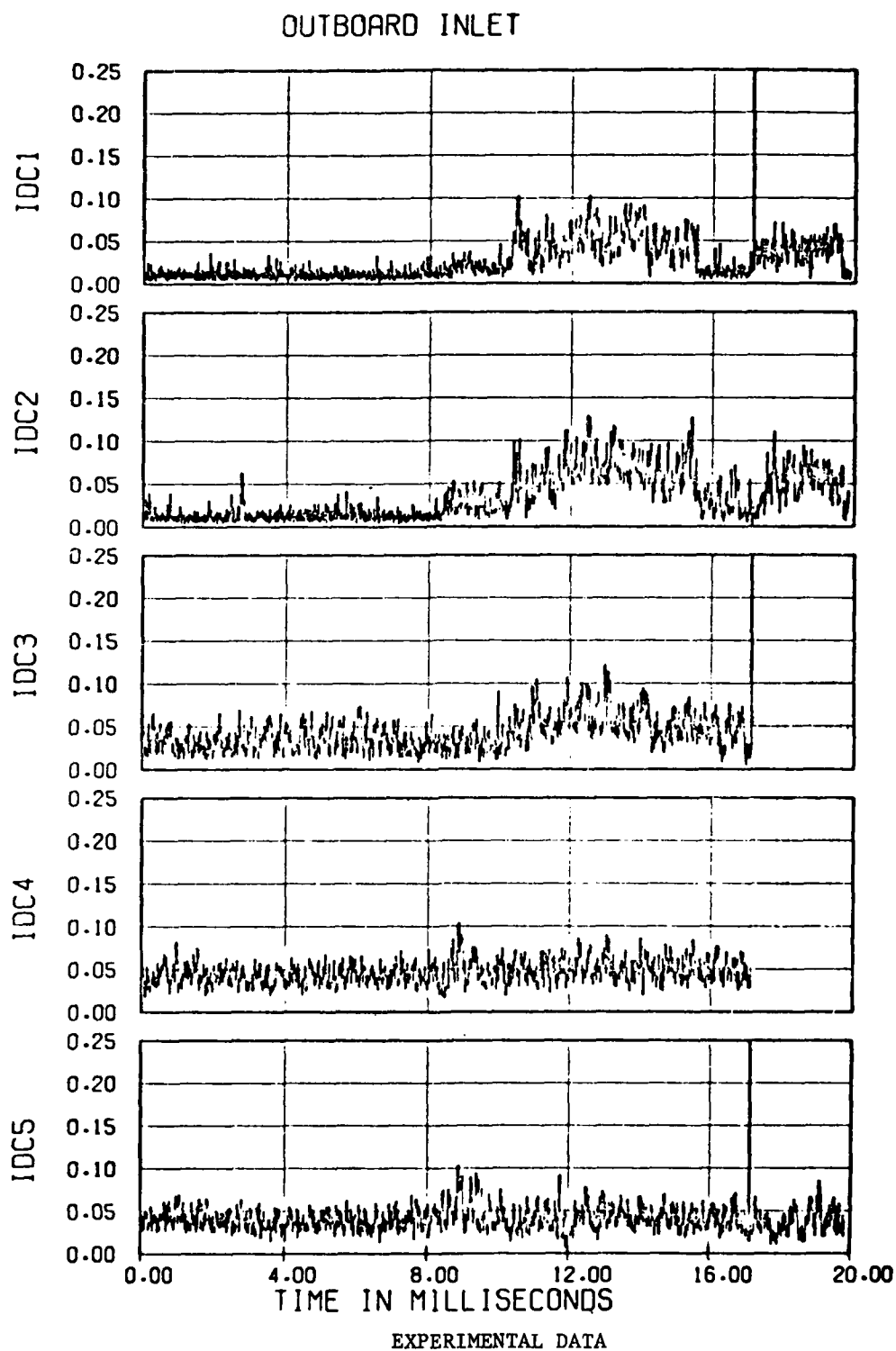
Figure 5.16a. Circumferential distortion.
