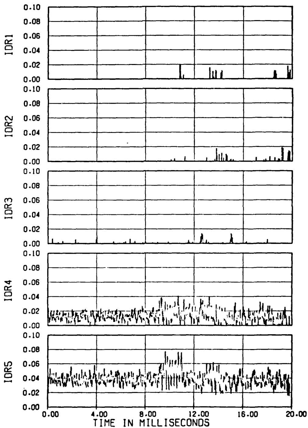
Figure 5.18b. Radial distortion.
