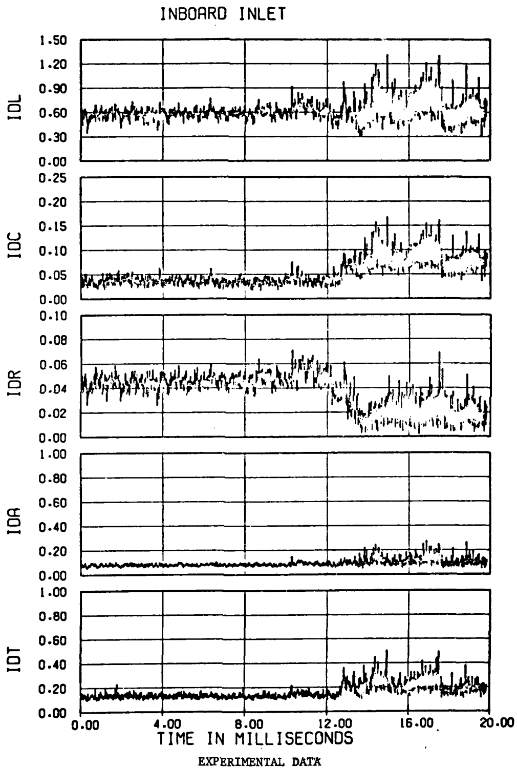
Figure 5.21c. Overall distortion.
