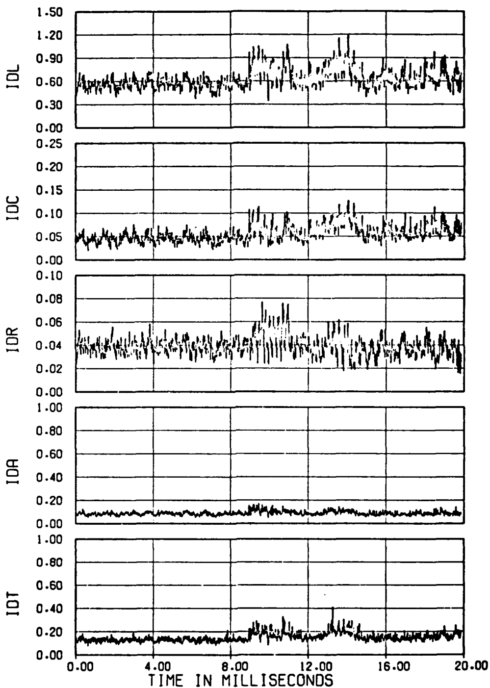
Figure 5.18c. Overall distortion.
