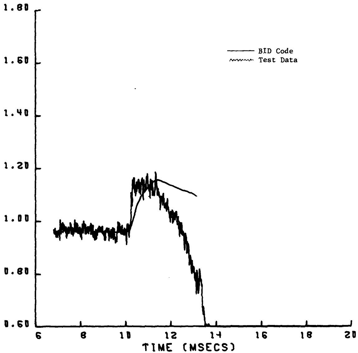
Figure 5.15f. Transducer 2830.
