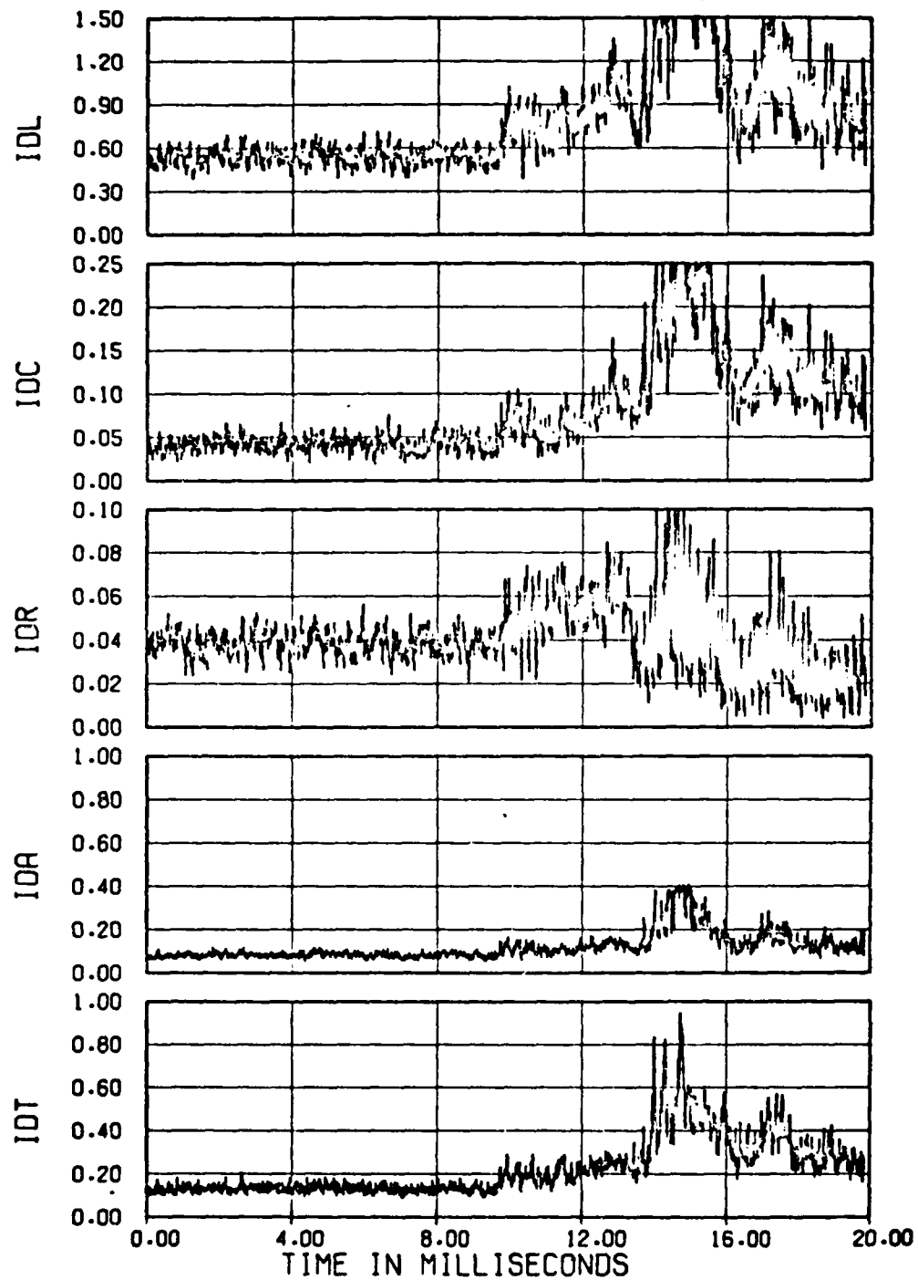
Figure 5.20c. Overall distortion.
