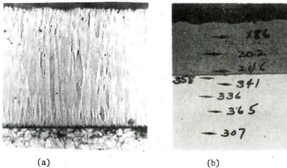
Figure 4. (a) Transverse section of a typical tantalum coating (X200). (b) Microhardness profile.
