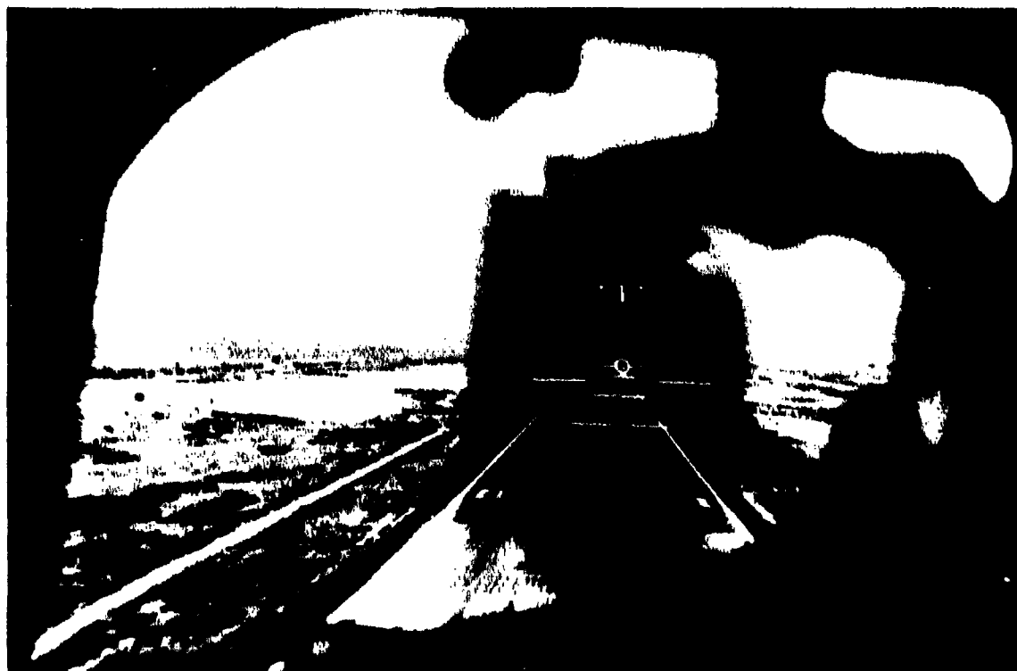
PILOT'S VIEW OF HEAD-UP DISPLAY DURING APPROACH TO OAKLAND AIRPORT. Development of Category III landing system in DC-9 Series 30, May 1967. Experimental installation used for manual touchdown or for monitoring automatic landing.
