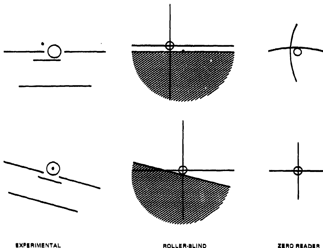
FIGURE 9. DISPLAYS OF COMMAND AND ATTITUDE USED IN EXPERIMENT 6. Commands for climbing turn to left shown above, satisfied commands shown below. Experimental display has one, and Roller-Blind two frameworks; Zero Reader only shows commands.
