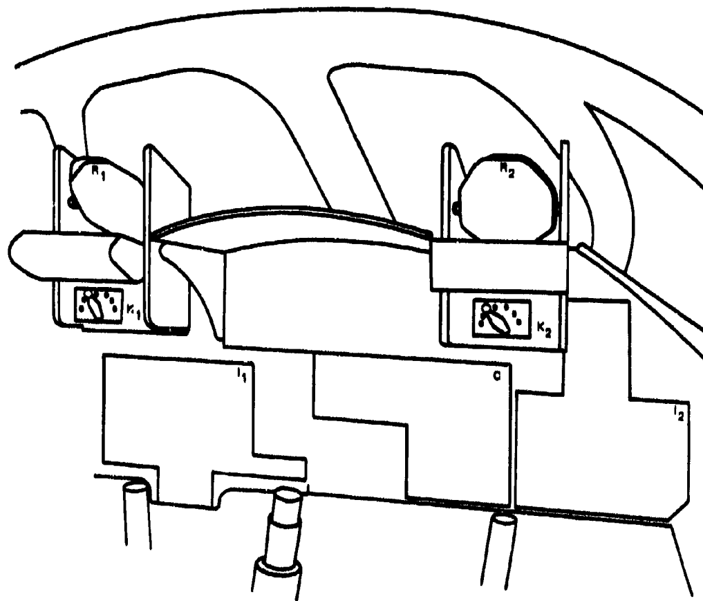
DISPLAY PRESENTED TO EACH PILOT THROUGH REFLECTOR PLATES R_1 , R_2 . CONTROL PANEL C WITH COMMAND INPUT FACILITY, BETWEEN INSTRUMENT PANELS I_1 , I_2 . POSITION OF REFLECTORS VARIED BY KNOBS K_1 , K_2 .
