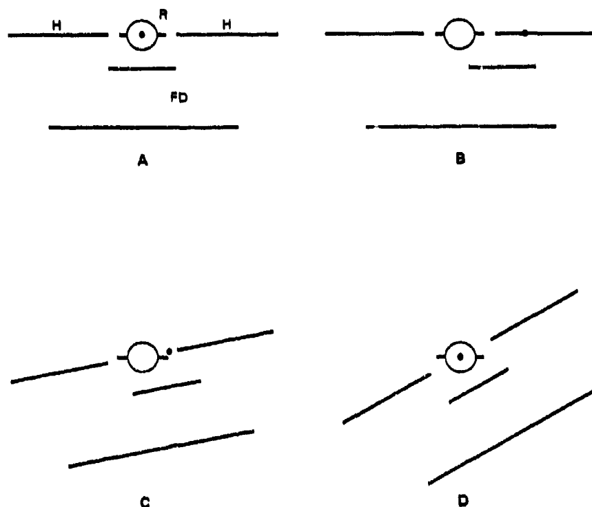
FIGURE 7. EXPERIMENTAL ATTITUDE AND COMMAND DISPLAY CONFORMING WITH FORWARD VIEW. (A) Aircraft reference R, Artificial Horizon HH, Flight Director FD. Azimuth command (B) partially satisfied (C) fully satisfied (D). Note movement of director index dot along horizon.
