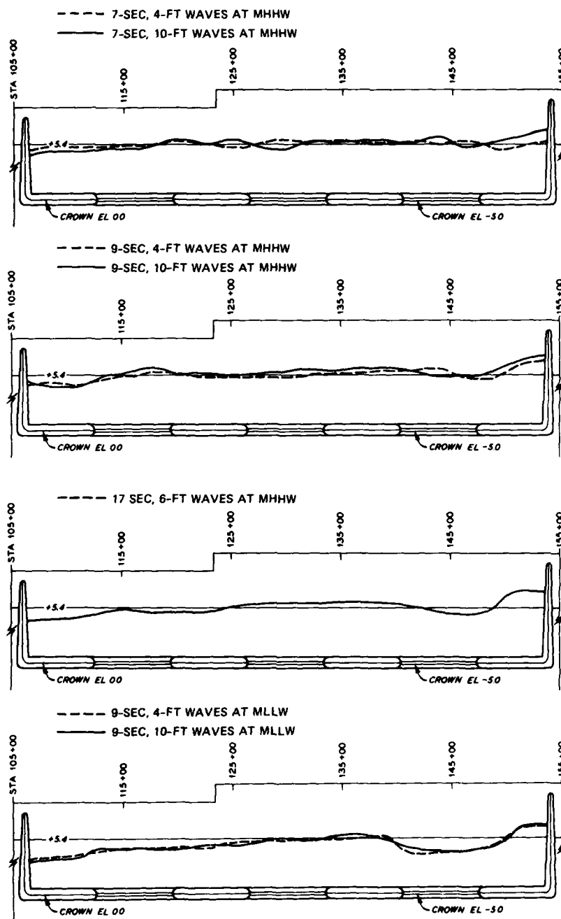
PLAN 14 MOVABLE-BED TRACER TESTS RESULTANT SHORELINE FOR WAVES FROM SOUTH WITH COAL FEED
