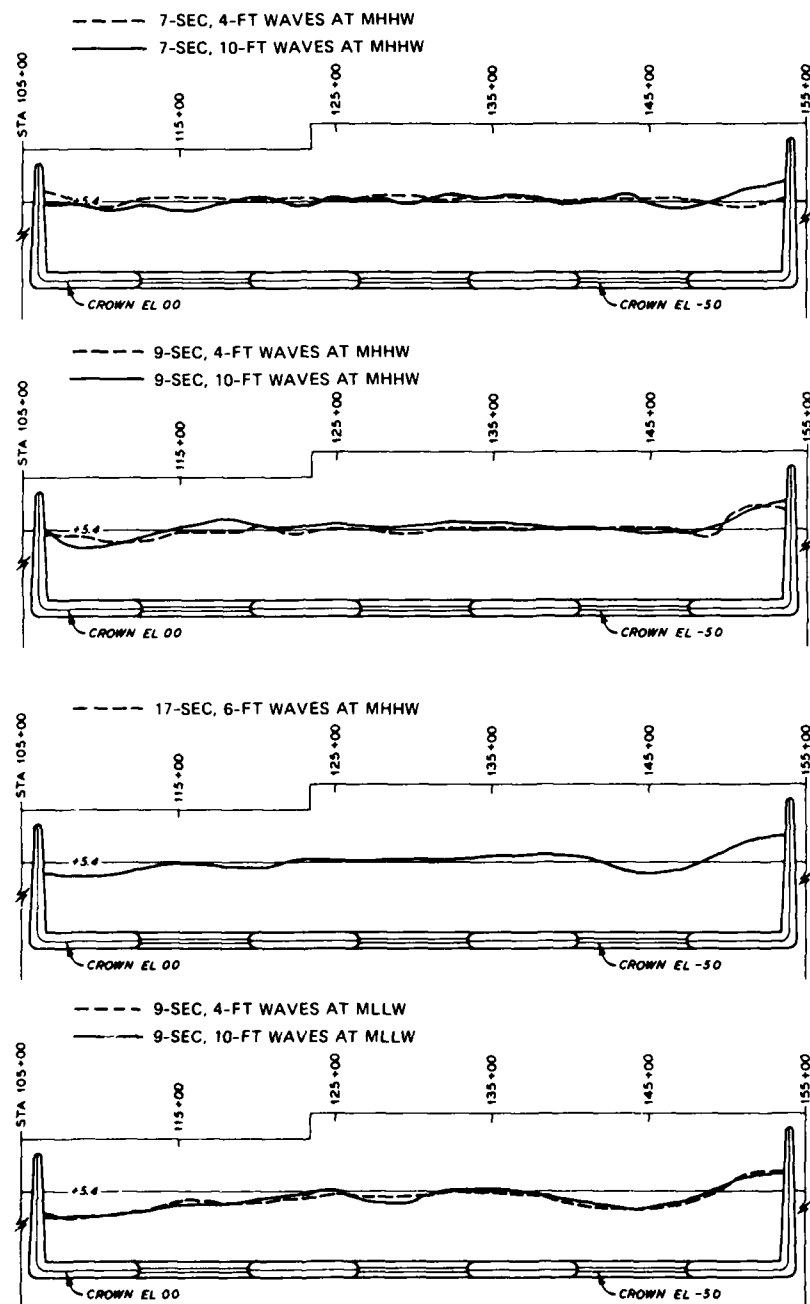
PLAN 14 MOVABLE-BED TRACER TESTS RESULTANT SHORELINE FOR WAVES FROM SOUTH WITHOUT COAL FEED
