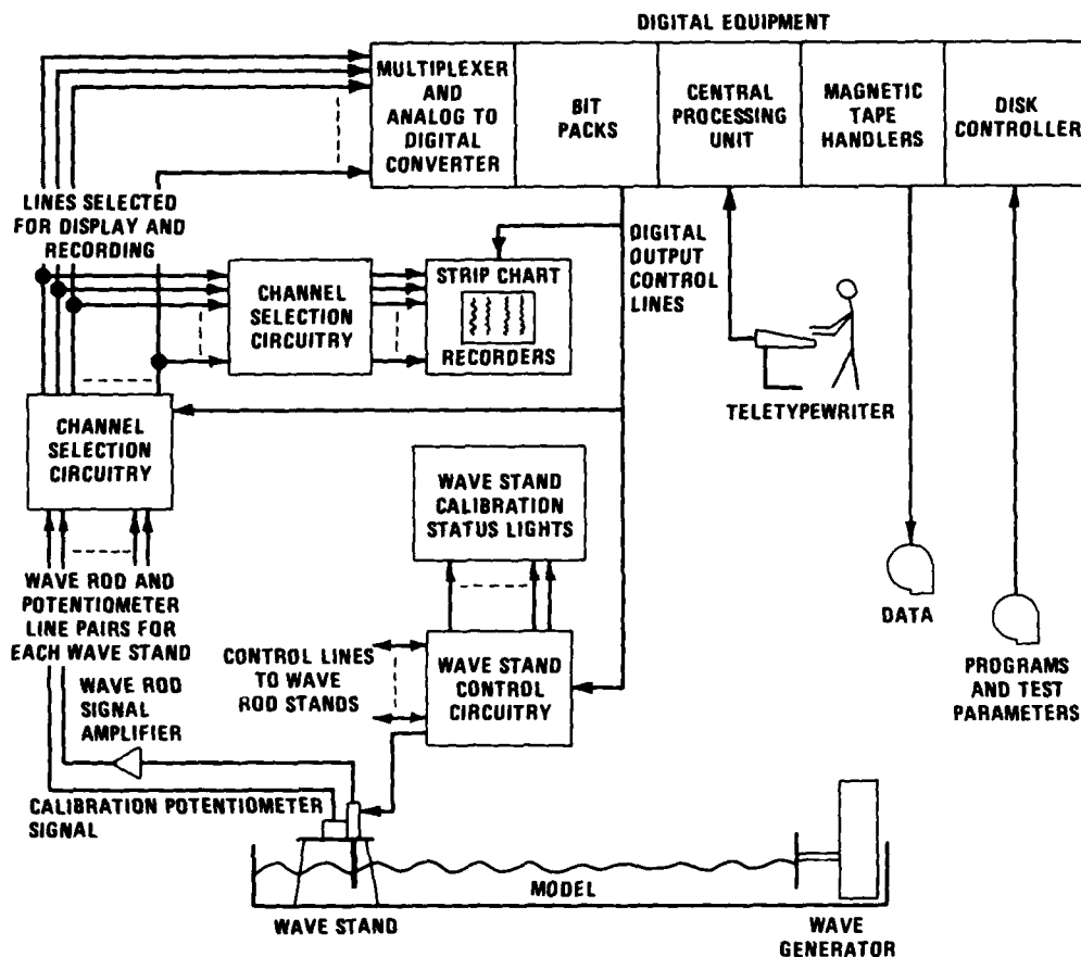
Figure 7. Automated Data Acquisition and Control System
