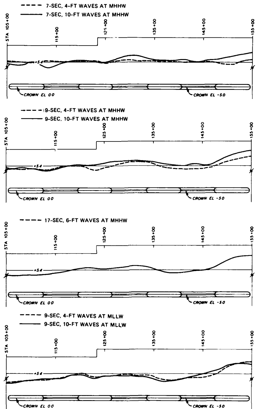
PLAN 13 MOVABLE-BED TRACER TESTS RESULTANT SHORELINE FOR WAVES FROM SOUTH WITH COAL FEED
