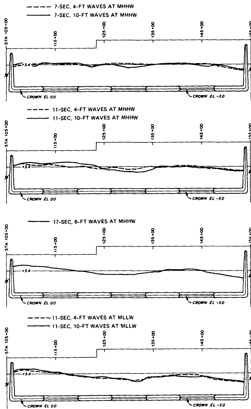
PLAN 14 A MOVABLE-BED TRACER TESTS RESULTANT SHORELINE FOR WAVES FROM WEST EXTENDED TEST WAVE DURATION
