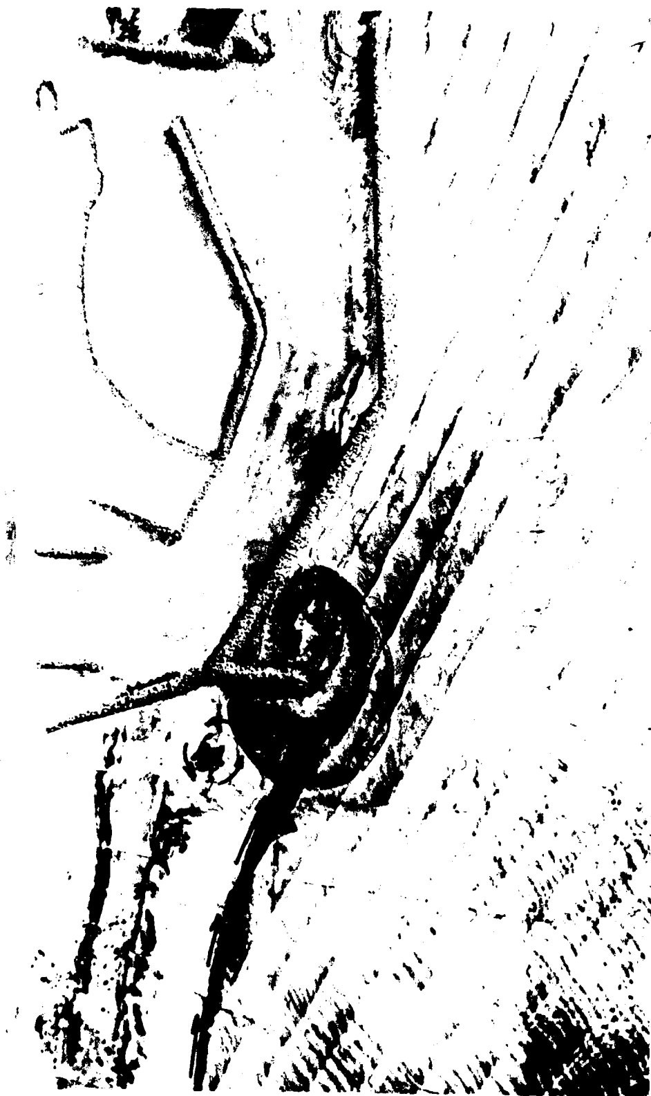
Photo 53. Typical tracer movement for Plan 62 resulting from 7-sec, 10-ft waves from northwest at mllw
