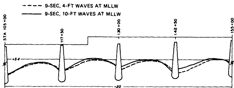
PLAN 6 MOVABLE-BED TRACER TESTS RESULTANT SHORELINE FOR WAVES FROM SOUTH
