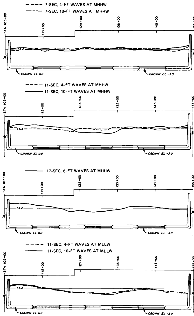
PLAN 14 MOVABLE-BED TRACER TESTS RESULTANT SHORELINE FOR WAVES FROM WEST EXTENDED TEST WAVE DURATION
