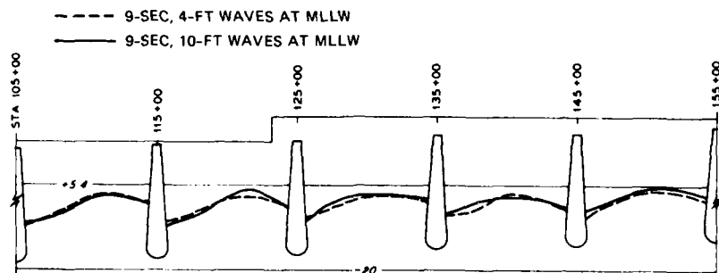
PLAN 9 MOVABLE-BED TRACER TESTS RESULTANT SHORELINE FOR WAVES FROM SOUTH WITHOUT COAL FEED
