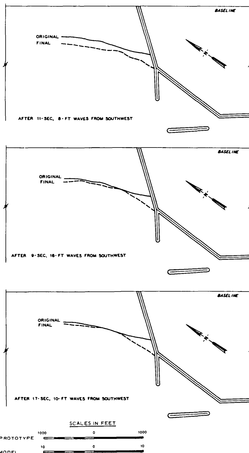
Figure 11. Shoreline plots for Plan 38C, waves from southwest at mhhw
