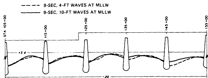
PLAN 9 MOVABLE-BED TRACER TESTS RESULTANT SHORELINE FOR WAVES FROM SOUTH WITH COAL FEED
