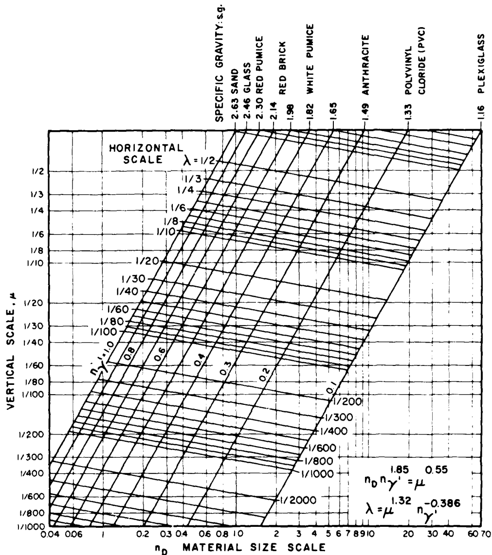
Figure 8. Graphical representation of model law (Noda 1971)
