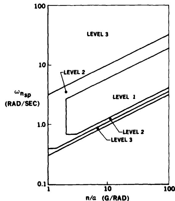
FIGURE 2-5. MIL-F-8785B SHORT-PERIOD FREQUENCY CRITERION
