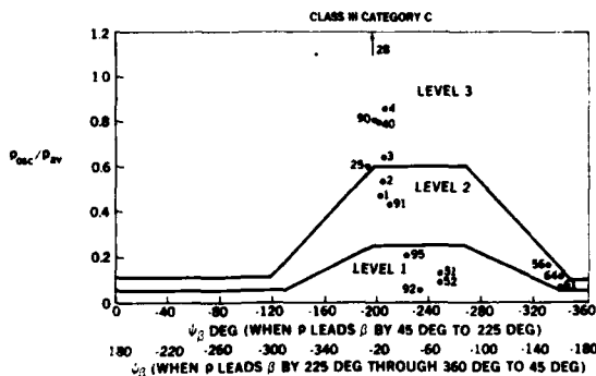
FIGURE 1-2. ROLL RATE OSCILLATIONS
