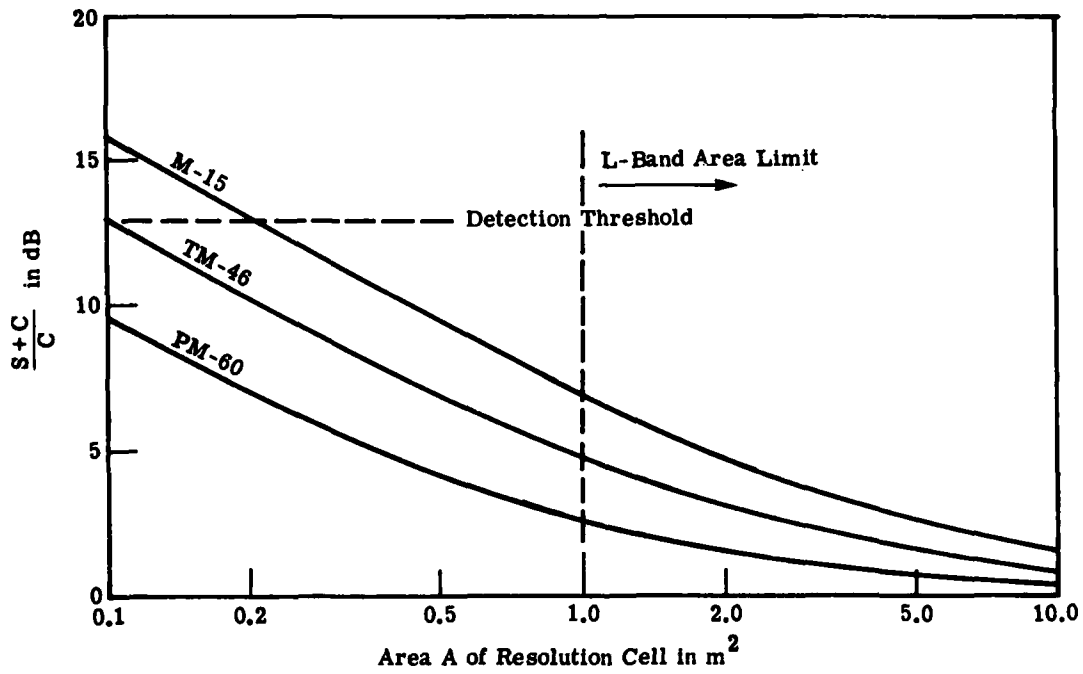
FIGURE 16. \frac{S+C}{C} VERSUS A , \sigma_0^0 = 0.01
