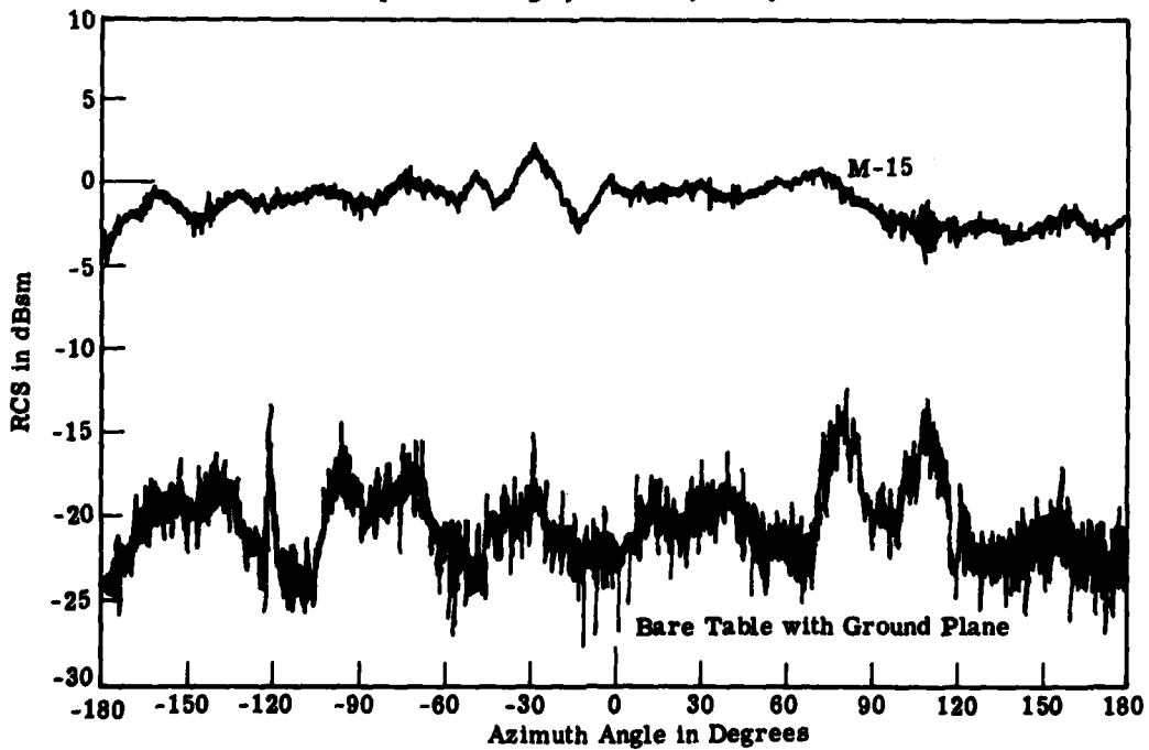
FIGURE 27. RCS OF M-15 ON METAL GROUND PLANE. Vertical Polarization, 22° Depression Angle, Chart 22, 9 May 1979.
