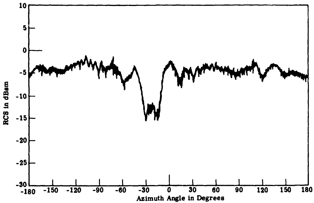
FIGURE 26. RCS OF TM-46 ON METAL GROUND PLANE. Vertical Polarization, 22° Depression Angle, Chart 21, 9 May 1979.
