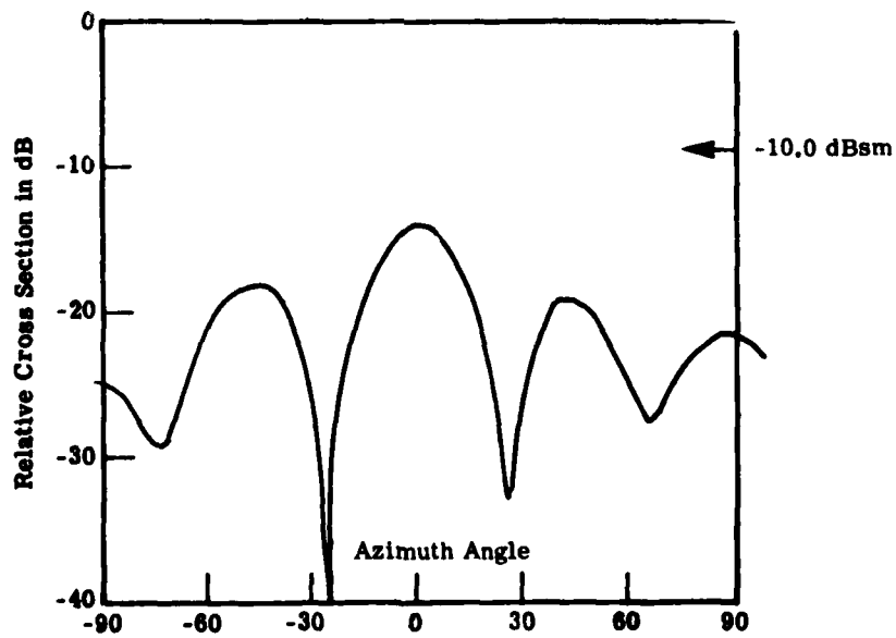
(b) Simulated PM-60, 1.2 GHz, Vertical Polarization
