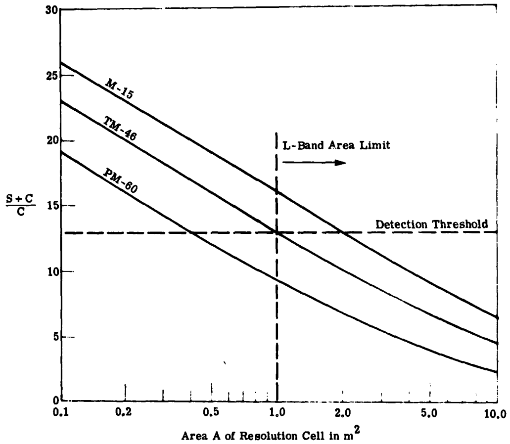
FIGURE 17. \frac{S+C}{C} VERSUS A, \sigma_0^0 = 0.001
