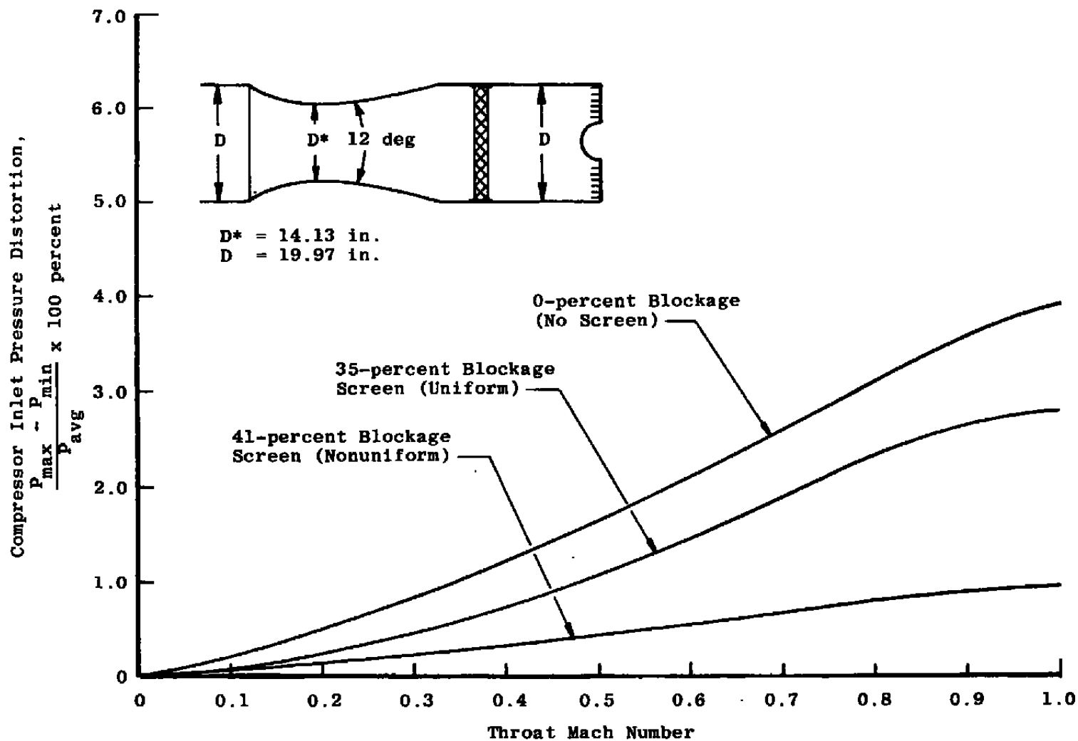
Figure C-7. Engine face total-pressure distortion (Ref. 17) (98 percent of flow area).
