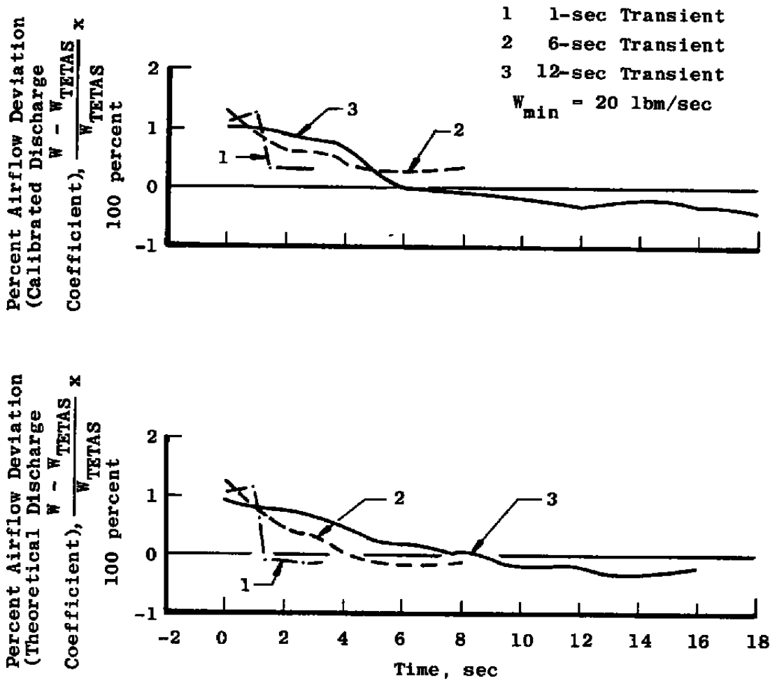
b. Deviation from TETAS airflow Figure 20. Concluded.
