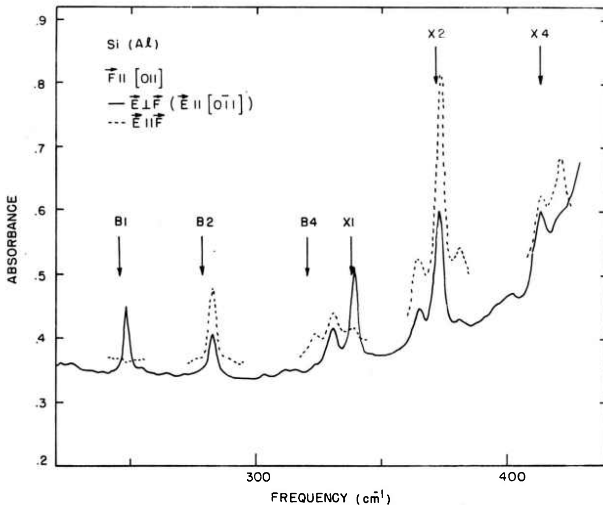
Figure C-5. The absorption spectrum of Al-doped silicon under [110] uniaxial compression with the incident light along [001] . The inferred level splittings are also shown, with two inequivalent subsets of the centers represented in two separate-level diagrams.
