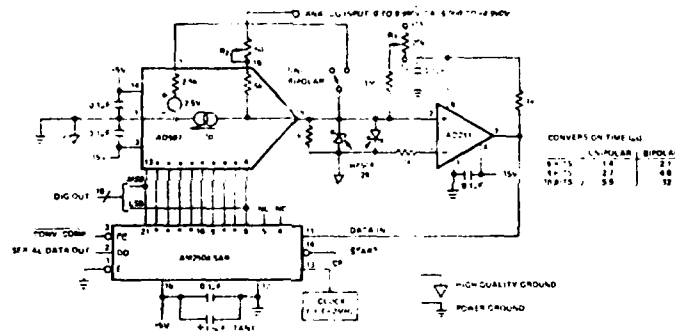
Figure 12. Fast Precision Analog to Digital Converter
