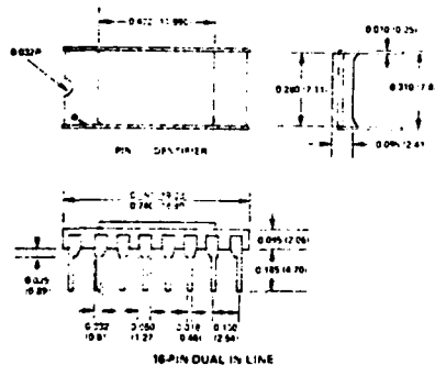
OUTLINE DIMENSIONS Dimensions shown in inches and (mm).
