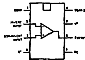
Dual-In-Line
