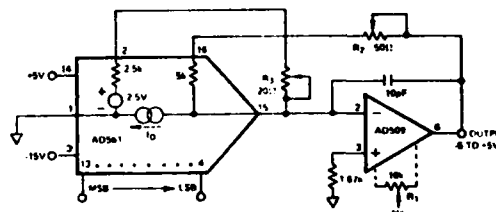
Figure 6. \pm 5 V Buffered Bipolar Voltage Output
