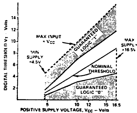
Figure 1. Digital Threshold Vs. Positive Supply
