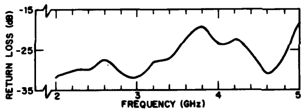
(b) Return loss
