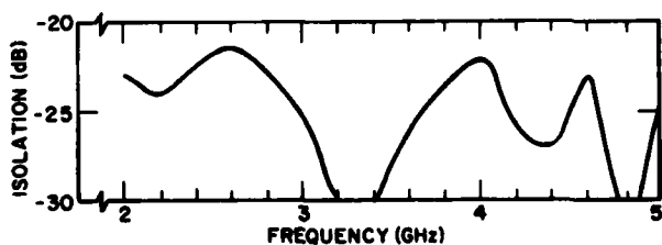
Fig. 8 - Microstrip/slotted-ground-plane coupler performance
