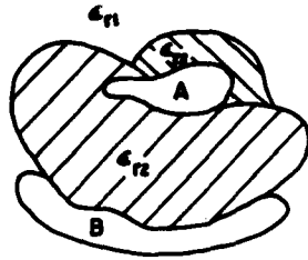
Fig. 1 — Cross section of an inhomogeneously loaded transmission line
