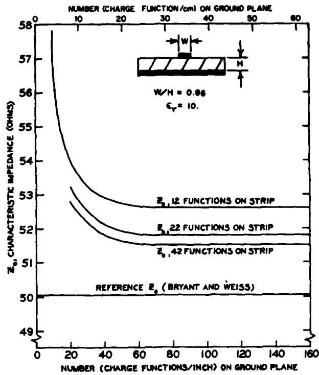
Fig. 2 - Convergence of computed microstrip impedance
