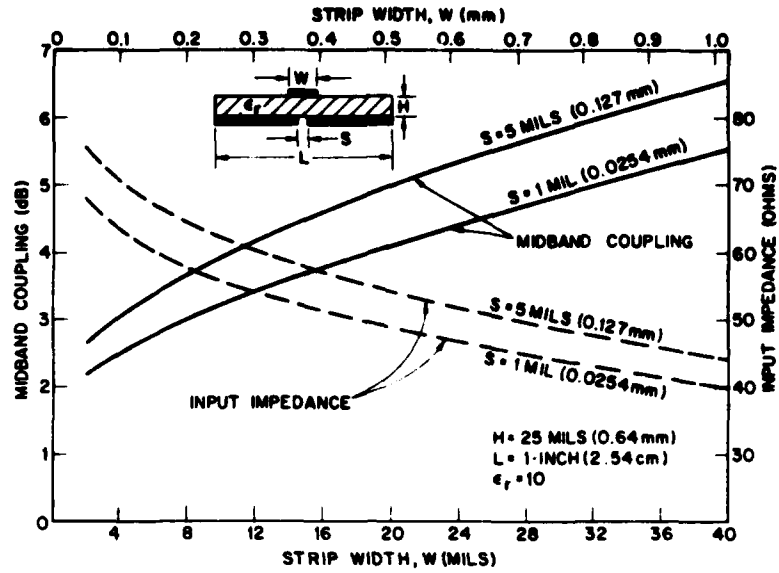
Fig. 4 — Midband coupling and input impedance for microstrip/slotted-ground-plane configuration
