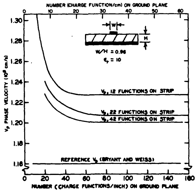
Fig. 3 - Convergence of computed microstrip phase velocity
