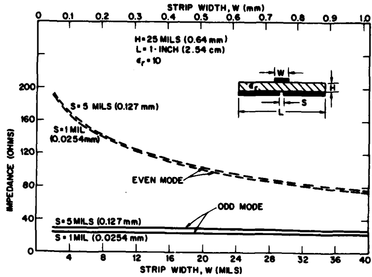
Fig. 6 — Even- and odd-mode impedances for microstrip/slotted-ground-plane configuration
