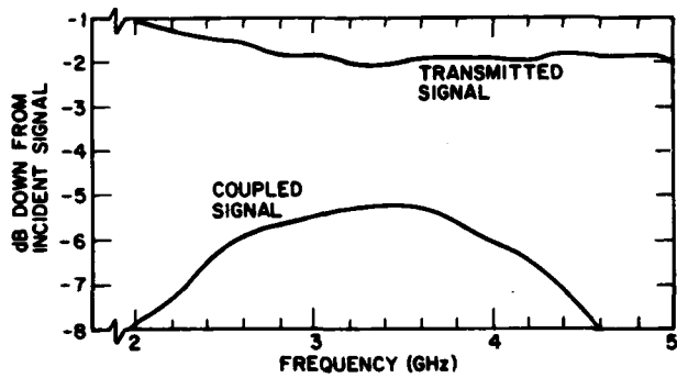
(a) Coupled and transmitted signals
