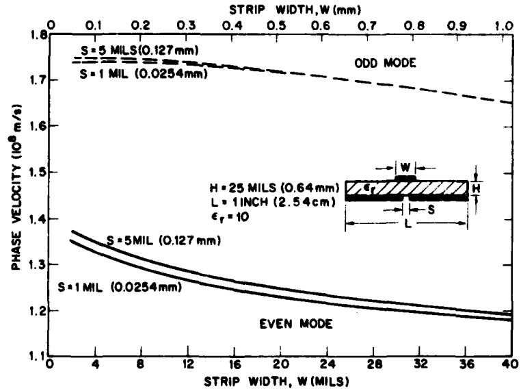
Fig. 5 — Even- and odd-mode-phase velocities for microstrip/slotted-ground-plane configuration
