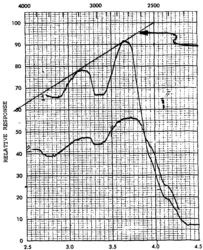
FIGURE 2-3. Responsivity vs. Wavelength for Photoconductive HgCdTe Detector Utilized in the 2 Micron Receiver (232°K)
