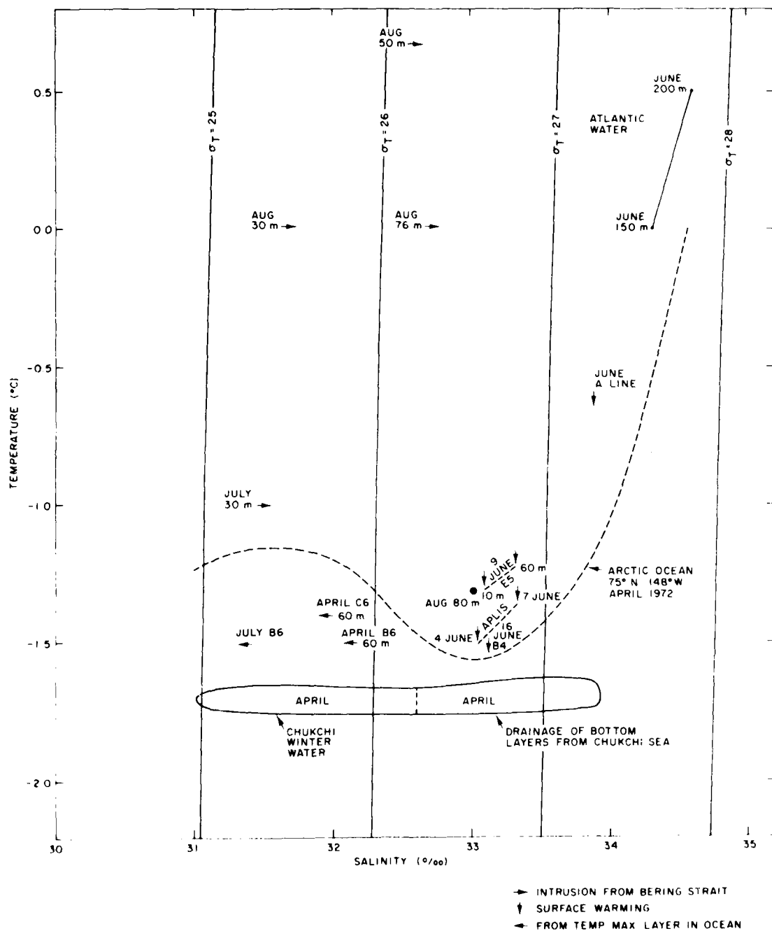
Figure 4b. Temperature-salinity diagram for the principal water masses encountered during summer 1977.
