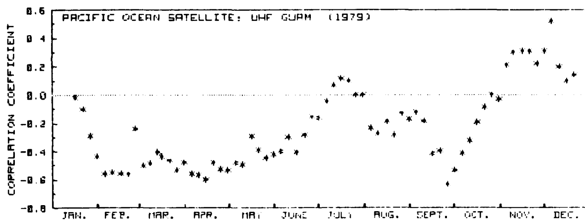
Figure 1. Cross correlations between total hours per night that scintillation fading exceeded 6 dB and the daily summed 3-hour Kp indices, using 30-day data samples.
