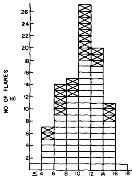
Figure 6. The Number of PCA Flares With a Given Comprehensive Flare Index (CFI). The flares in (b) were followed by subsequent events while those in (a) were not. The dashed vertical line is drawn for comparison with Figure 5. Data were not available for two events
