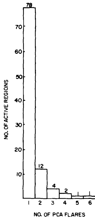
Figure 1. The Number of Solar Active Regions Generating a Given Number of PCA Parent Flares, 1955-1976 (Sample size = 133 events)
