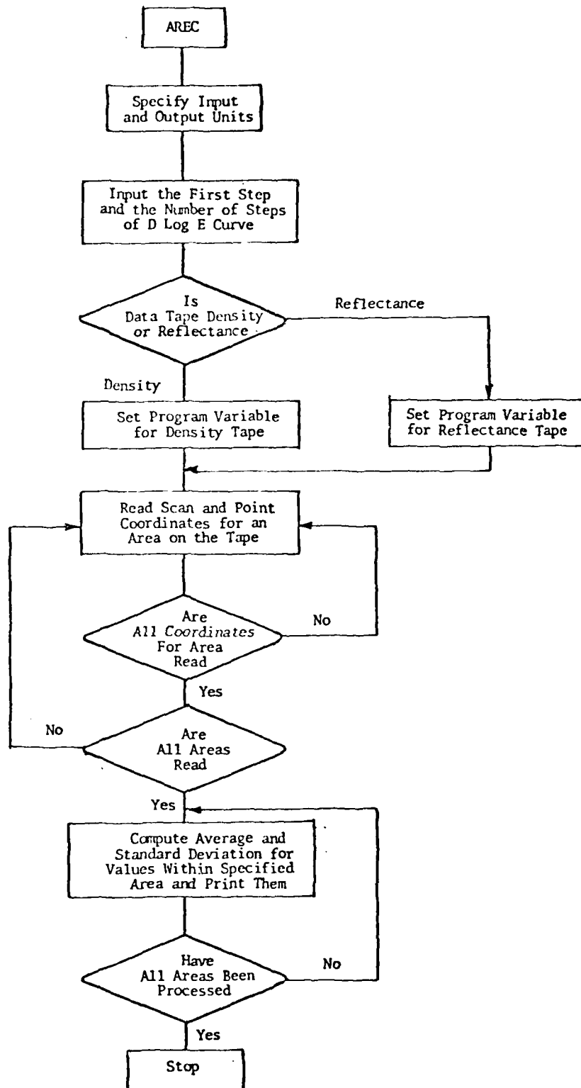
FIGURE B-2. PROGRAM AREC FLOW DIAGRAM
