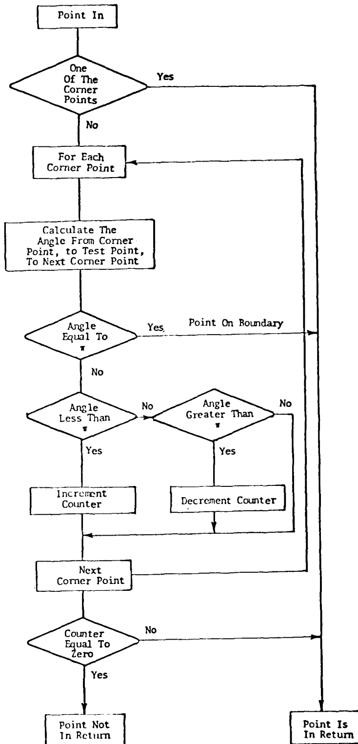
FIGURE B-4. SUBROUTINE NTIN FLOW DIAGRAM
