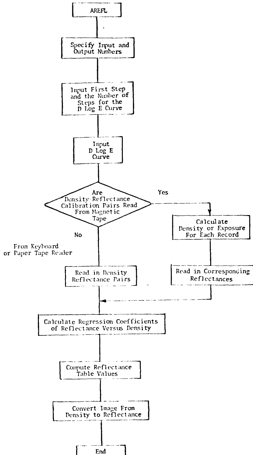
FIGURE B-1. PROGRAM AREFL FLOW DIAGRAM
