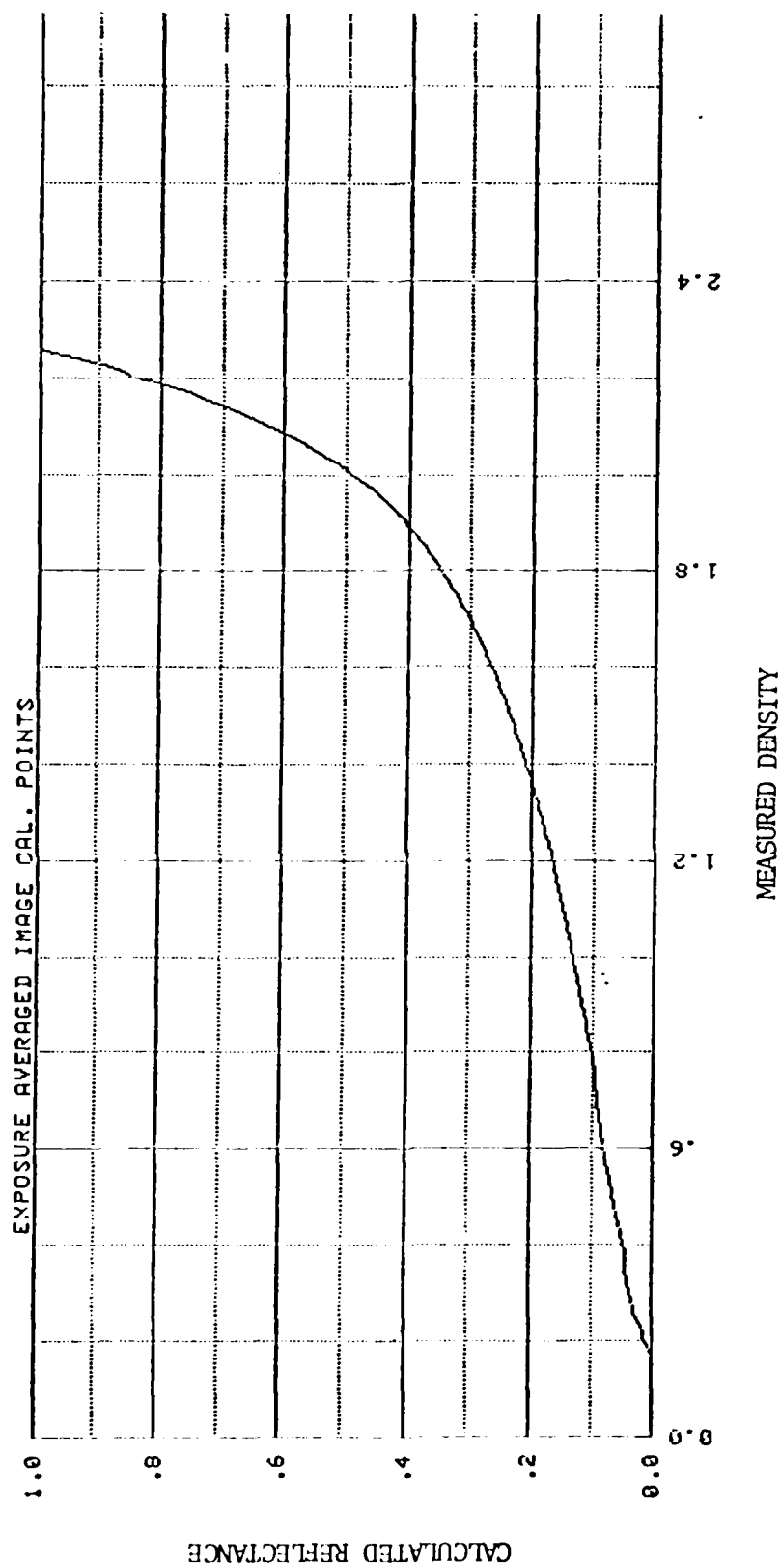
Figure 5-27 DENSITY TO REFLECTANCE CONVERSION FOR DIGITAL IMAGE CALIBRATION AREAS (LOW HAZE, EXPOSURE-AVERAGED)
