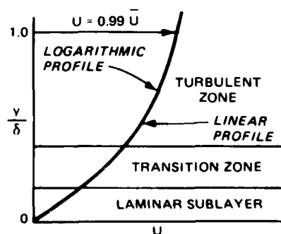
SMOOTH WALL FLOW
