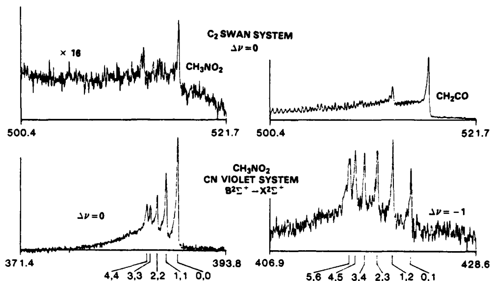
Fig. 10. Above : Spectra of the C 2 Swan emission ( \Delta v = 0 ) derived from ketene at 10 torr and nitromethane at 15 torr. Note the reduced intensity of the signal from nitromethane. Below : Spectra of the CN violet system emission ( \Delta v = 0 , \Delta v = -1 ) derived from nitromethane at 15 torr. Data are accumulated from 30 laser shots.
