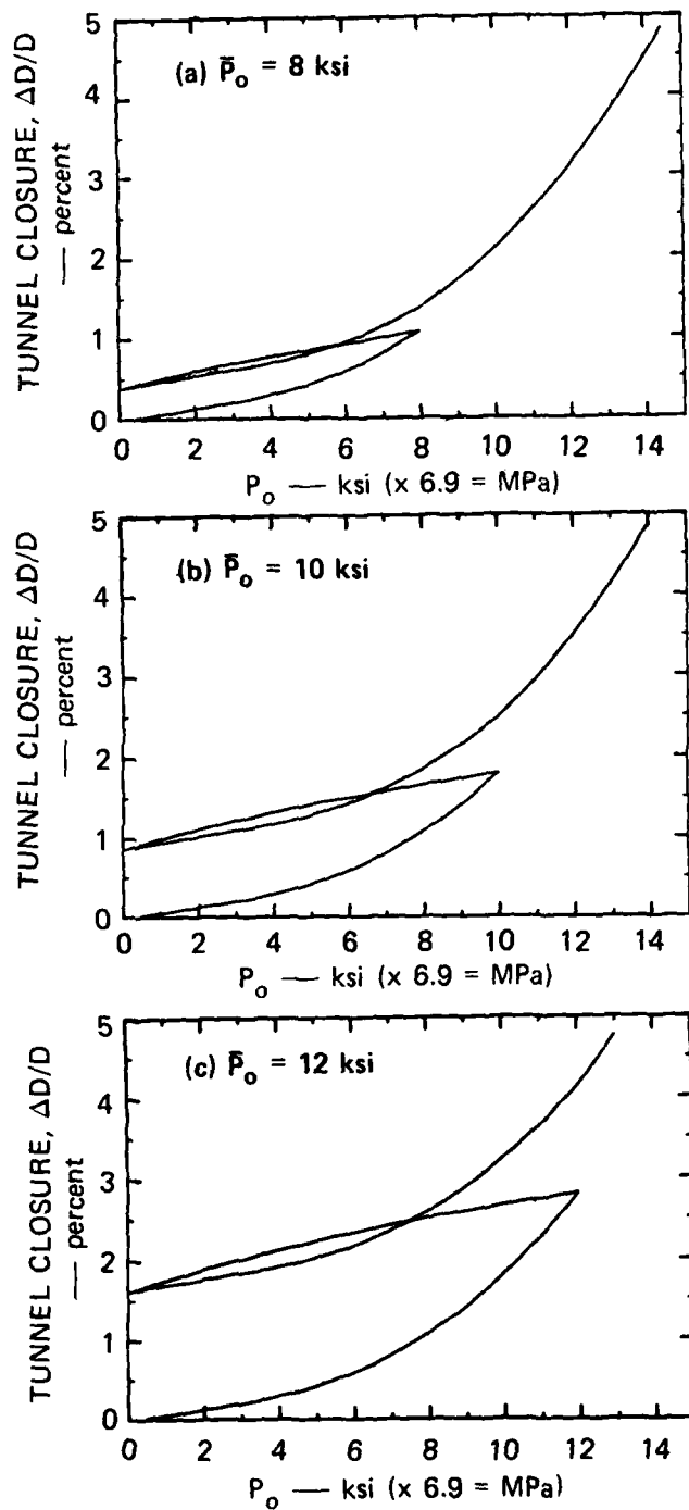
FIGURE 4.2 EFFECT OF \bar{P}_o ON RELOAD CLOSURE P_i = 0.5 ksi, \sigma_u = 4 ksi, N_\phi = 3 (1 ksi = 6.9 MPa)
