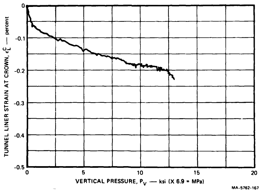
FIGURE A.58 TUNNEL LINER STRAIN AT CROWN VERSUS VERTICAL PRESSURE — TEST LSUX-20
