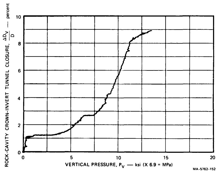
FIGURE A.43 ROCK-CAVITY CROWN-INVERT TUNNEL CLOSURE VERSUS VERTICAL PRESSURE — TEST LSUX-19
