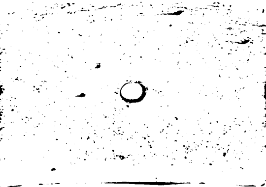
FIGURE 2.23 POSTTEST CROSS SECTIONS SHOWING DISTRIBUTION OF PORES IN HUSKY ACE ROCK-MATCHING GROUT
