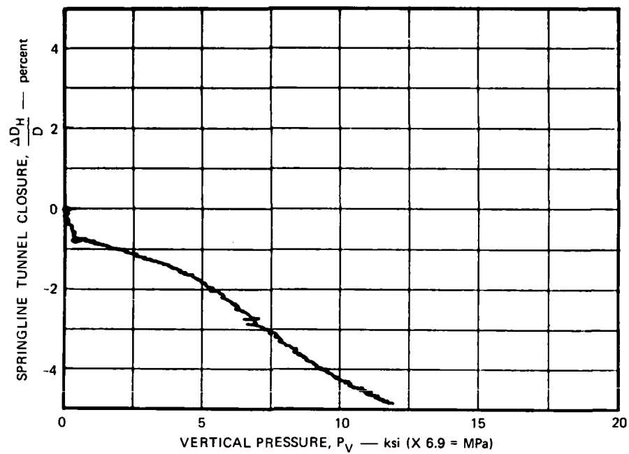
FIGURE A.13 SPRINGLINE TUNNEL CLOSURE VERSUS VERTICAL PRESSURE TEST LSUX-14
