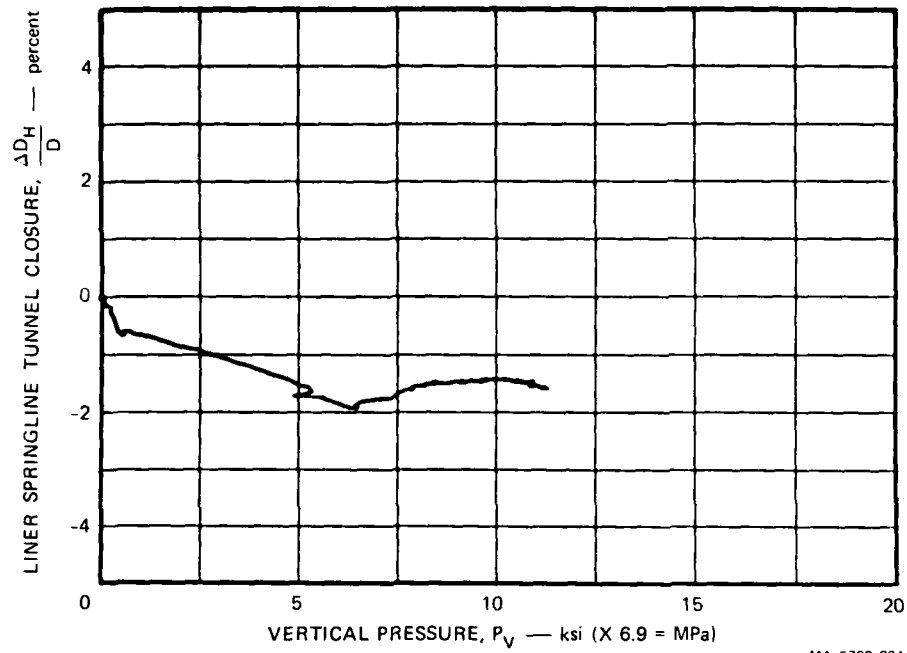
FIGURE A.95 LINER SPRINGLINE TUNNEL CLOSURE VERSUS VERTICAL PRESSURE — TEST LSUX-25
