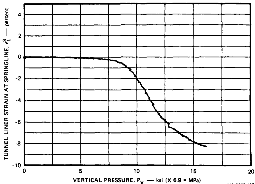
FIGURE A.88 TUNNEL LINER STRAIN AT SPRINGLINE VERSUS VERTICAL PRESSURE — TEST LSUX-24
