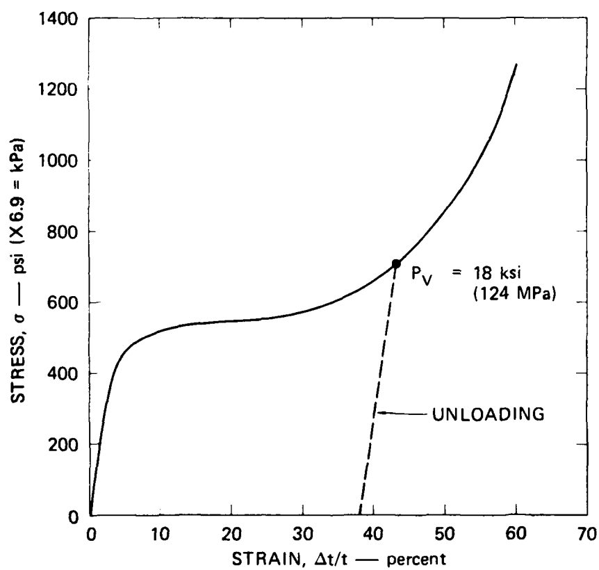
FIGURE 4.8 STRESS-STRAIN CURVE FOR UNIAXIAL STRAIN LOADING OF 13.2 lb/ft 2 (211 kg/m 3 ) POLYURETHANE FOAM \dot{\epsilon} = 3.3 \times 10^{-2} \text{ s}^{-1}
