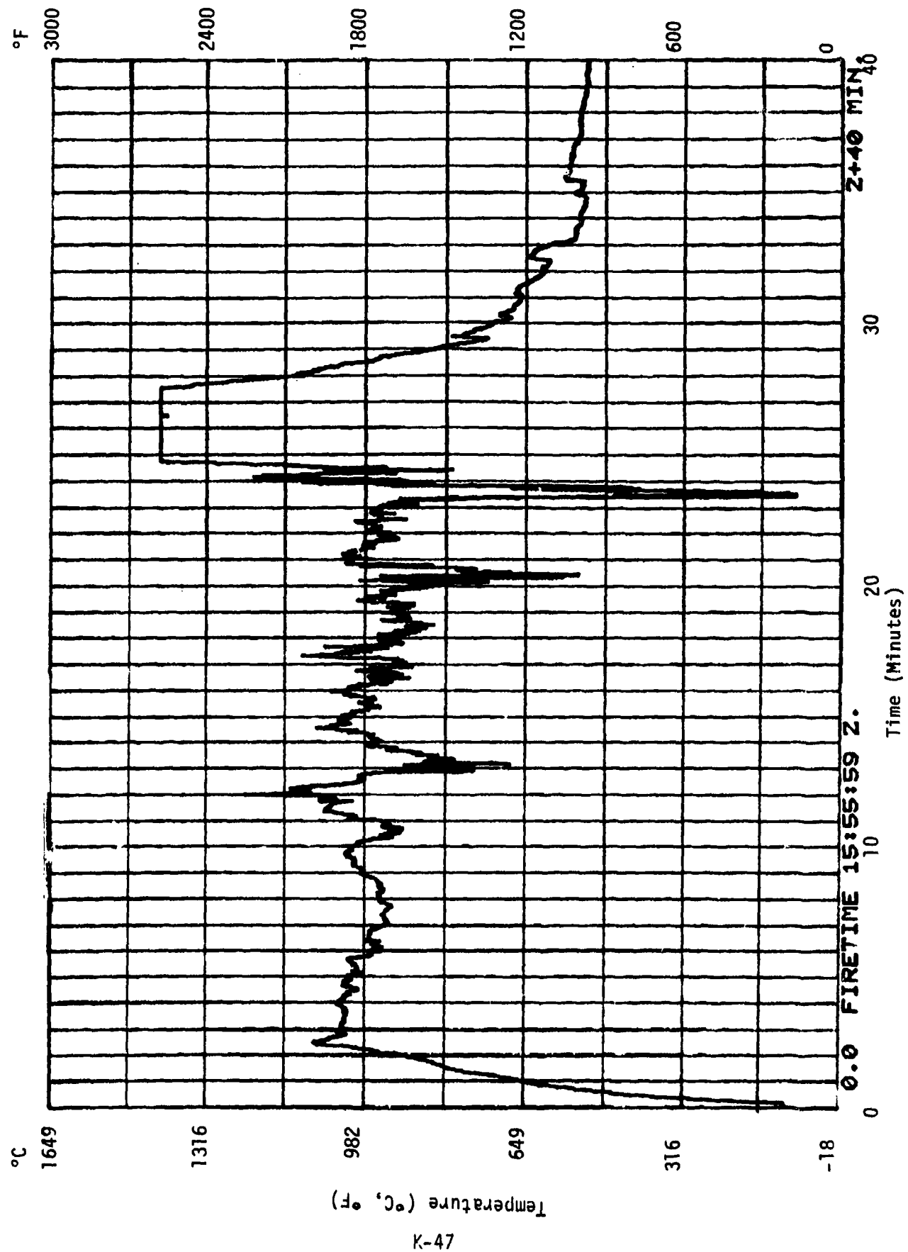
Figure K.42. Temperature Measurements for NASA Carbon Fiber Pool Fire Trial S-1, 15 November 1979, Thermocouple Number 8.
