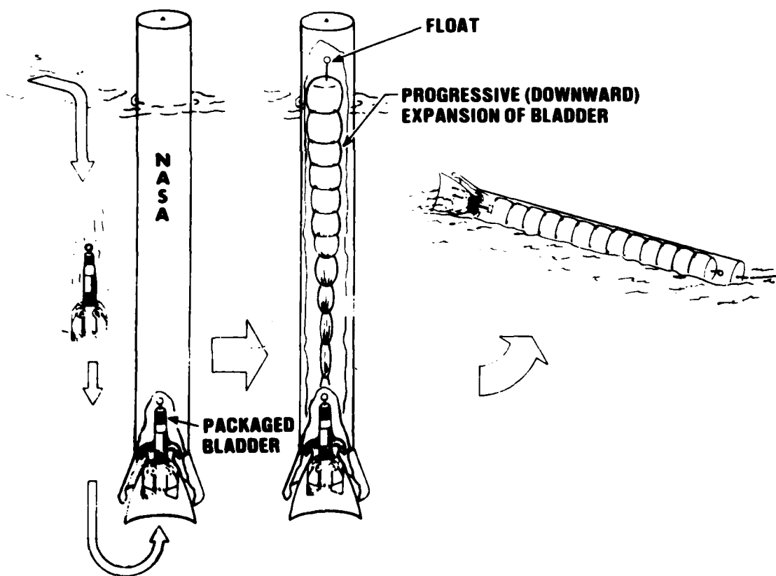
Figure 35. Inflatable bladder module.
