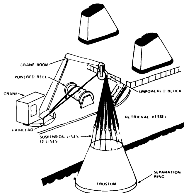
Figure 22. Unpowered block with powered reel.
