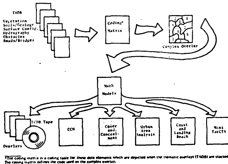
Figure 1. Synthesis process.
