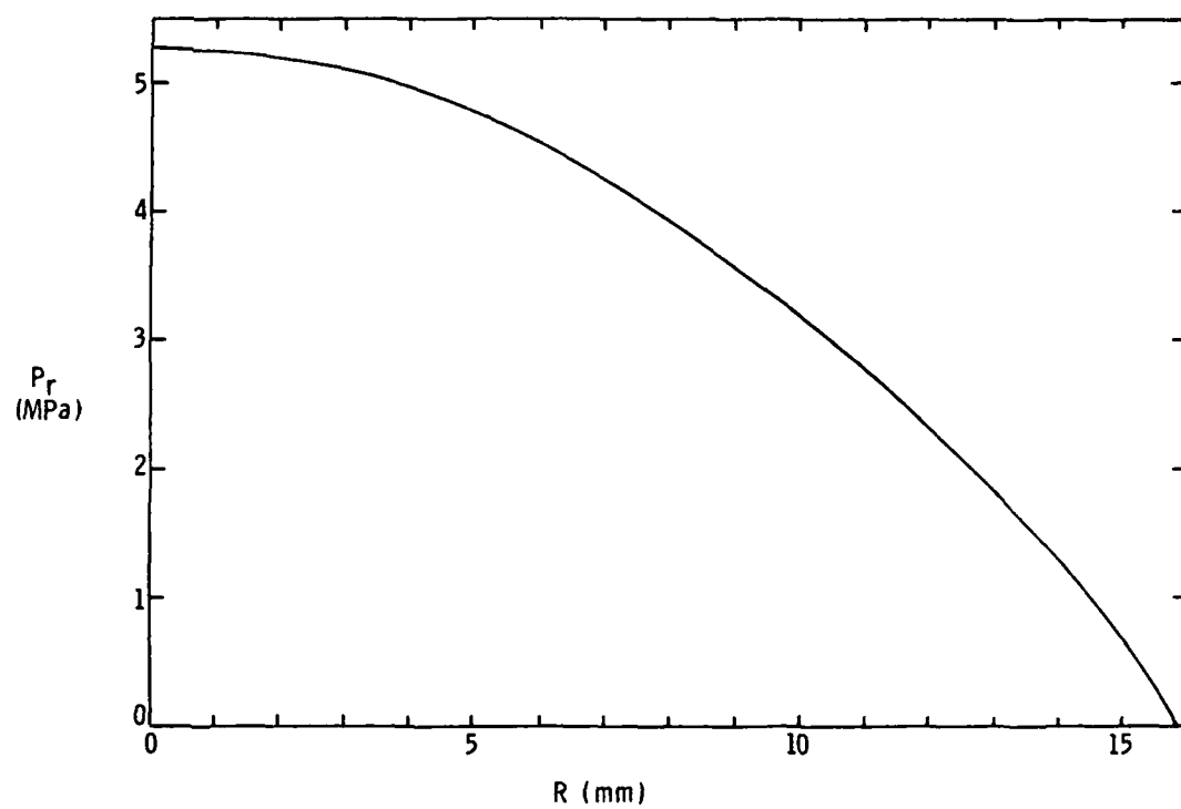
Figure 24. Predicted Pressure Distribution, P_s = 2.592 MPa, \dot{Q}_1'' = 3.785 MW/m 2 .
