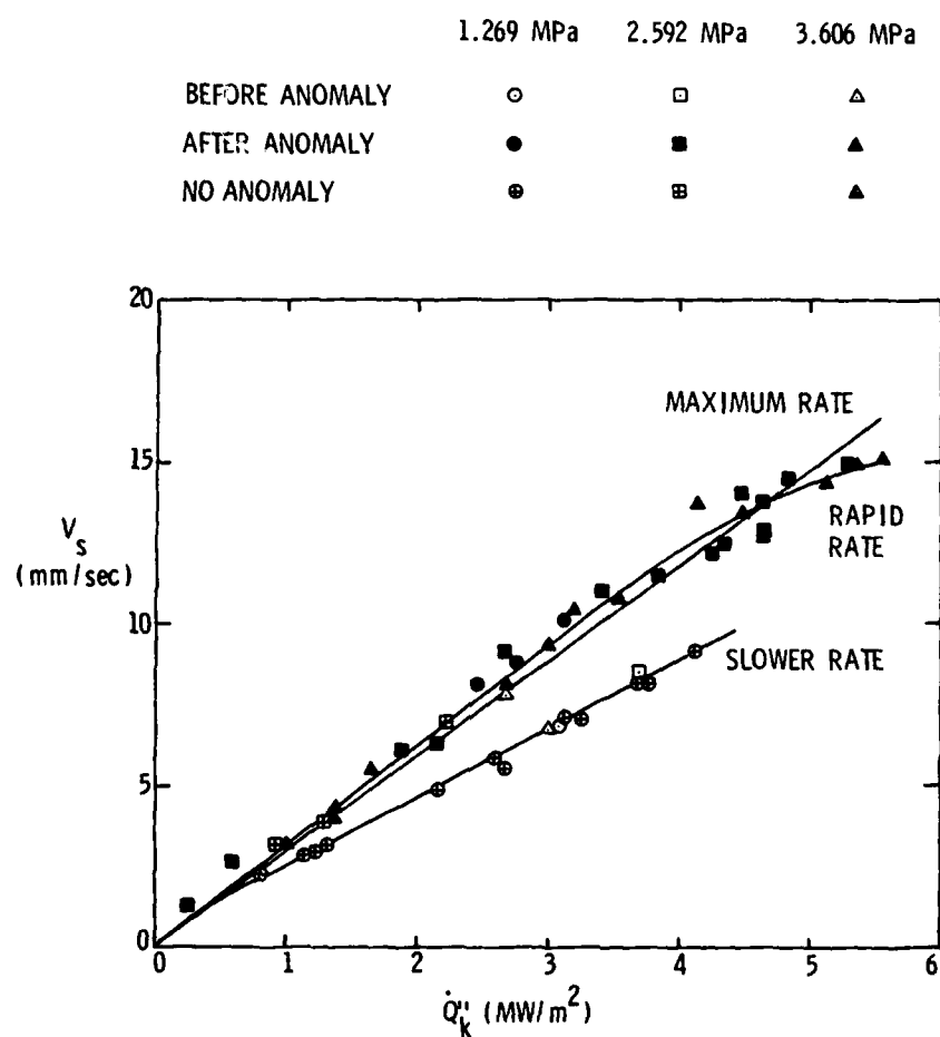
Figure 17. Experimental Results, V_s versus \dot{Q}_k'' .
