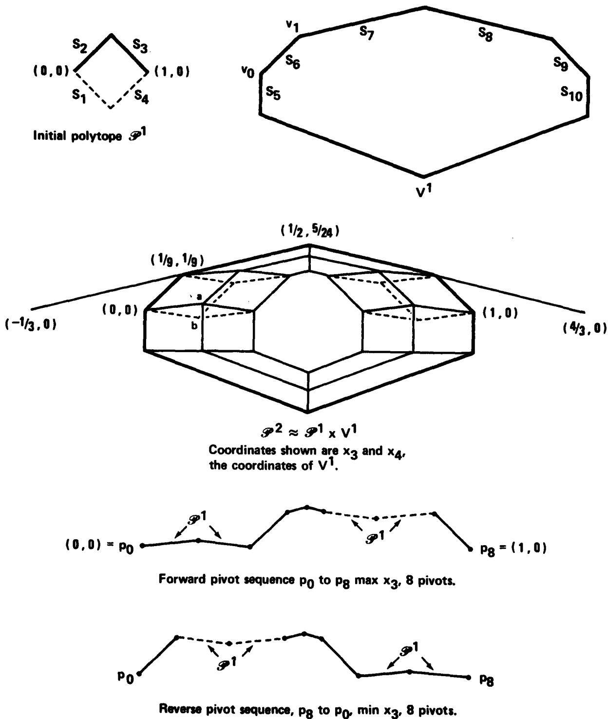
Figure 2: A modification of the Klee-Minty-Jeroslow construction.
