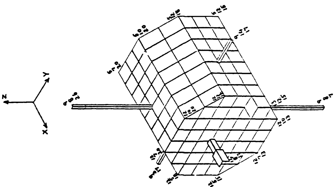
Figure 2. NASCAP 1-Grid Representation of SCATHA Satellite
