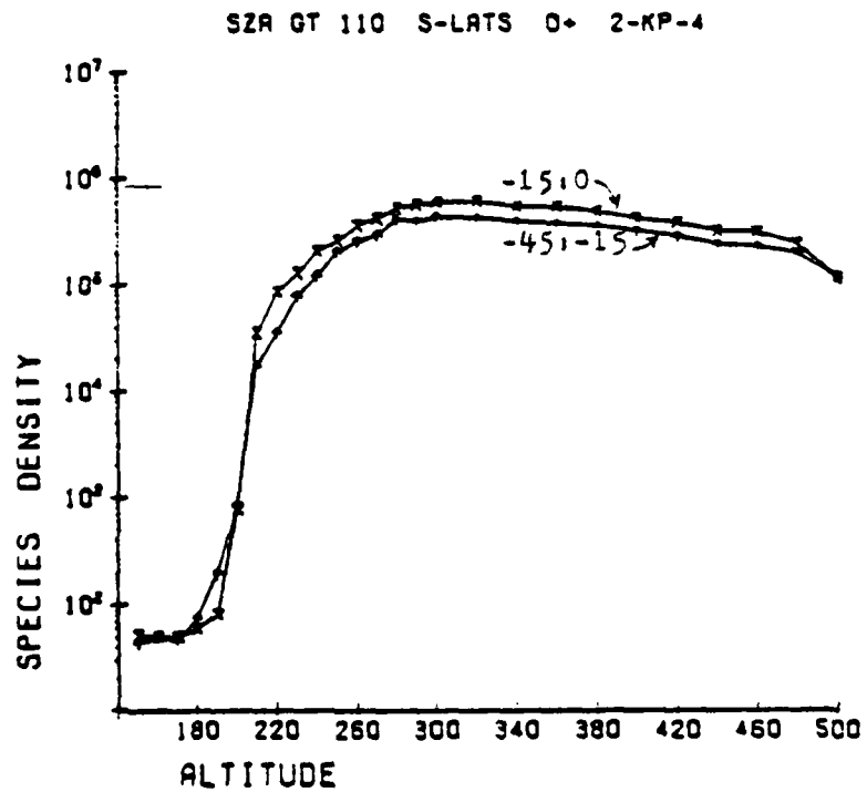
Figure 7. Latitudinal Parametric Profile Plots for O^+ at Night
