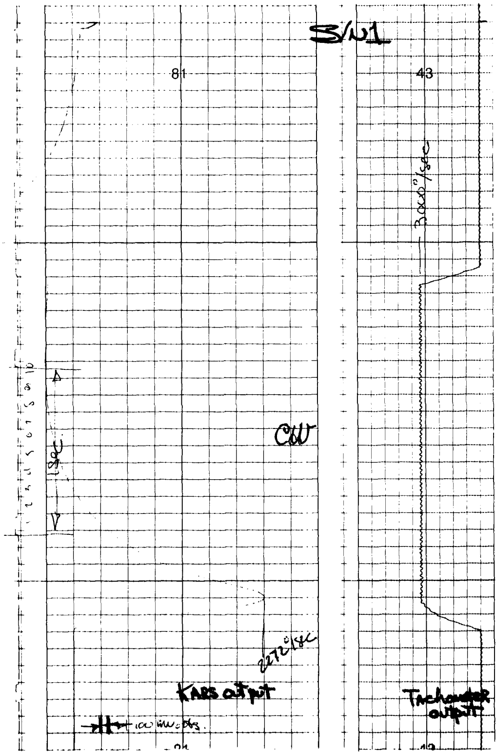
Figure 36. S/N 1 3000°/sec Step Input Response
