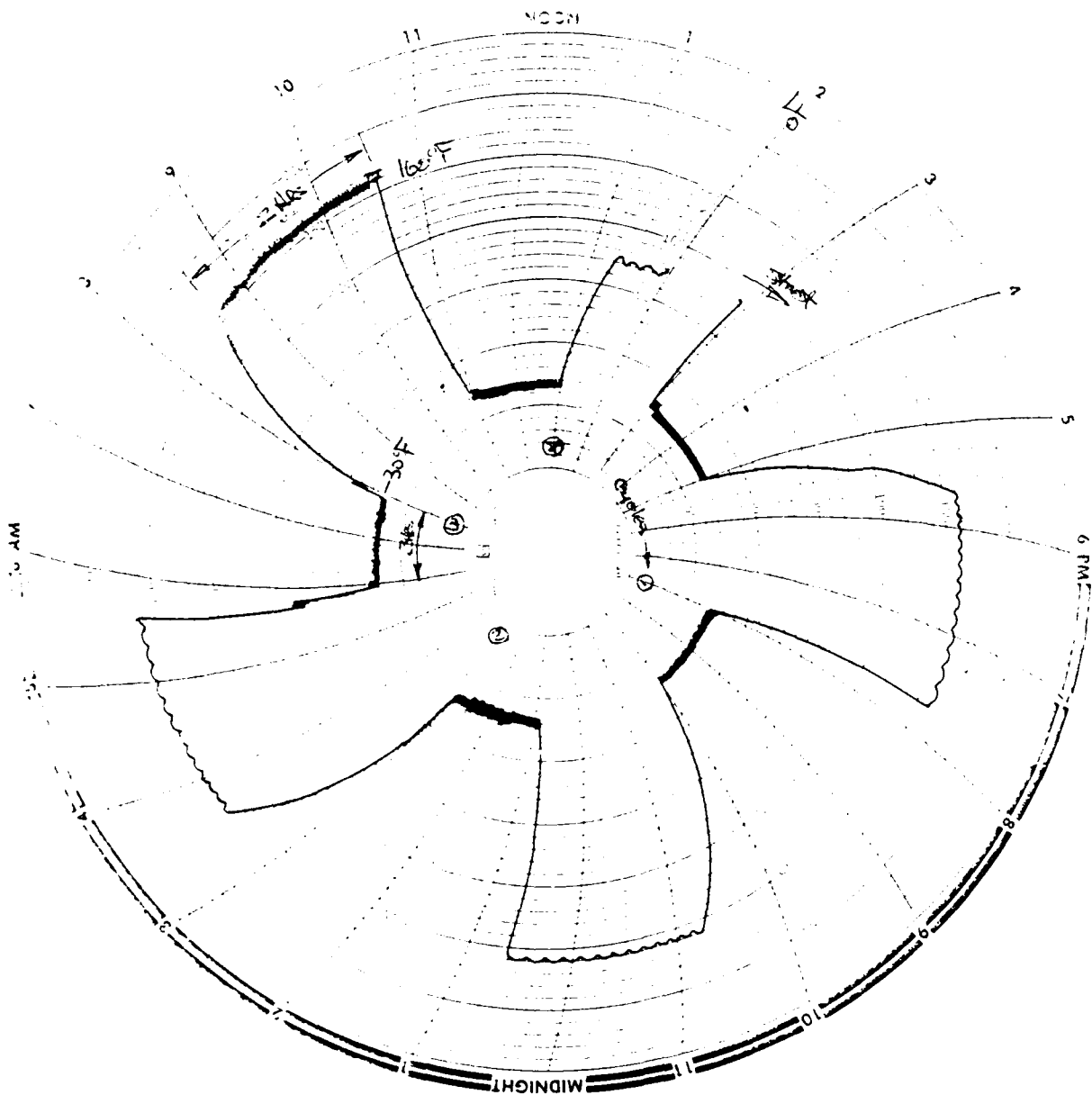
Figure 46. Environmental Temperature Cycle KARS
