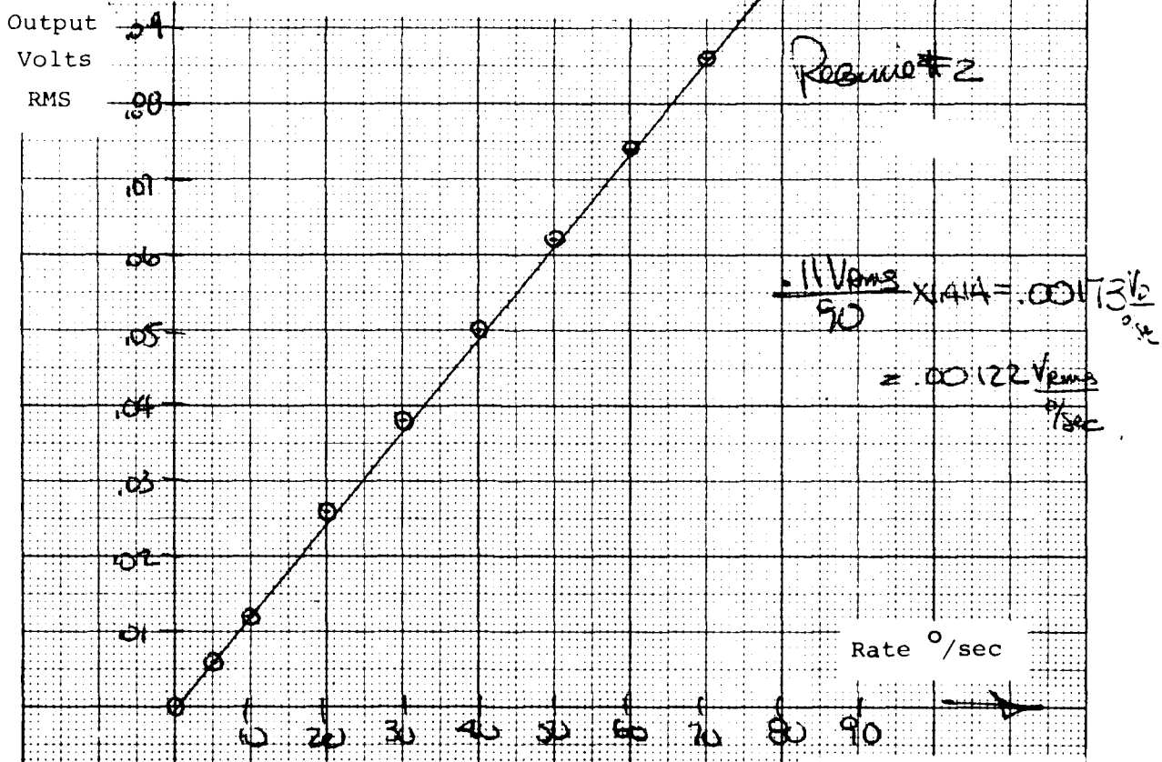
Figure 39. S/N 2 Regime #2 Scale Factor Plot
