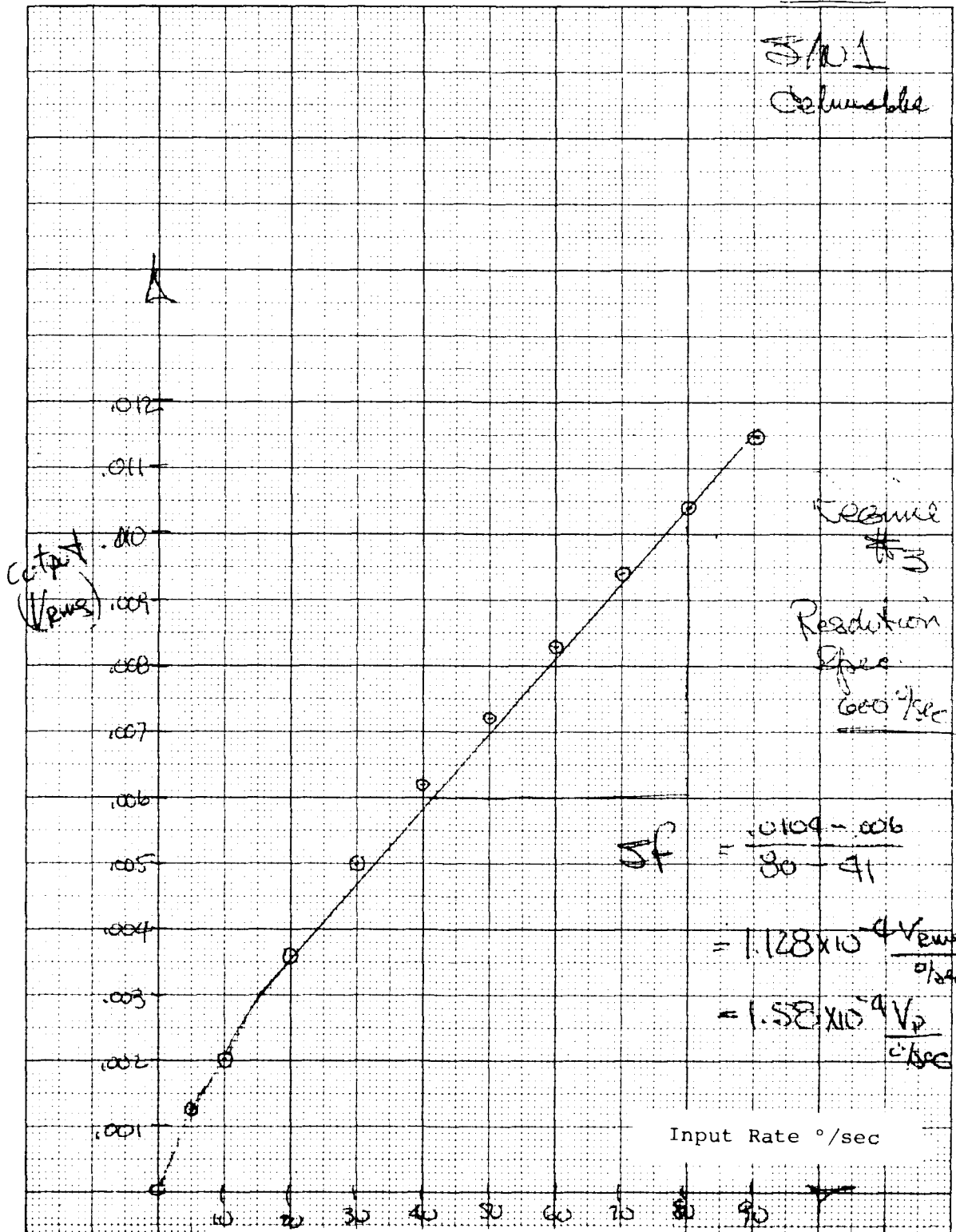
Figure 32. S/N 1 Regime #3 Scale Factor Plot
