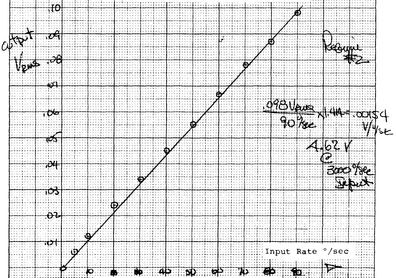
Figure 31. S/N 1 Regime #2 Scale Factor Plot
