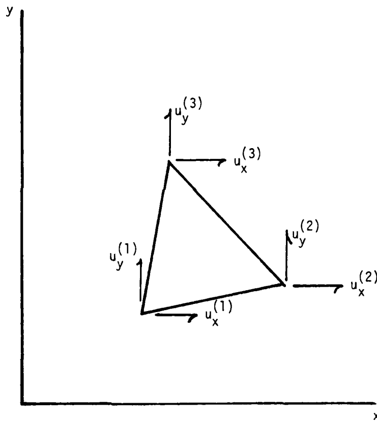
FIGURE 1 TRIANGULAR ELEMENT
