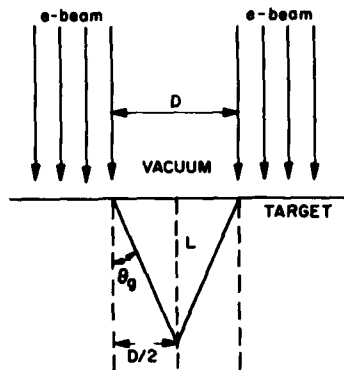
Fig. 9. Diagram depicts two e-beams, separated by a distance D , striking the target; the geometrical angle, \theta_g , and the undercutting length, L , are visually defined.
