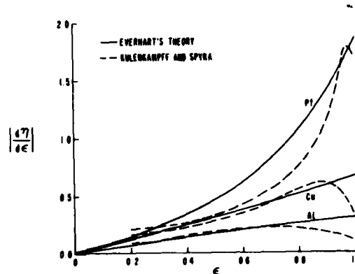
Fig. 3. Comparison of EDC's of Everhart's theory with those experiments obtained in ref. (6) for Al, Cu, and Pt.
