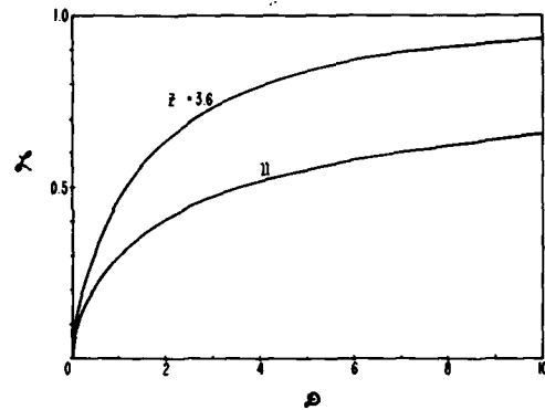
Fig. 10. Plot of reduced depth L , as a function of reduced separation, D , with average atomic number, Z , as a parameter.
