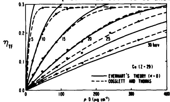
Fig. 7. Comparison of \eta_{TF} with experiment for Cu.
