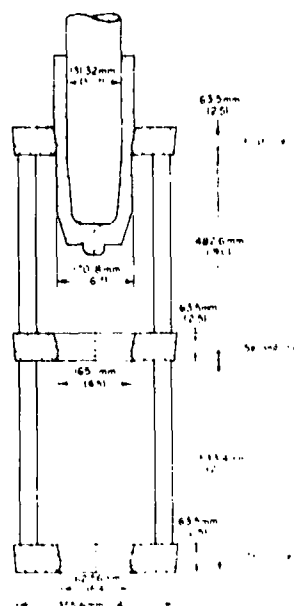
Figure 7. Schematic representation of hot drawing of 155 mm M107 shell.
