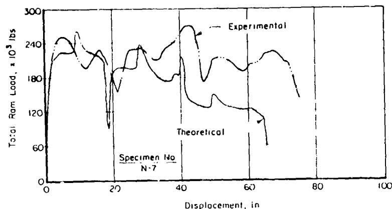
Figure 12. Theoretical and experimental load-displacement curves for cold hot drawing of M107 shell through conical dies for preform length = 342.9 mm (13.5 inch).
