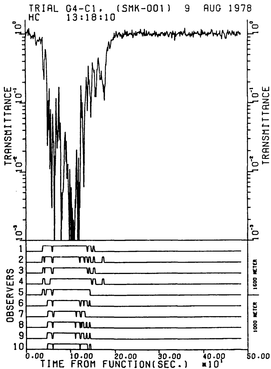
FIGURE 10. Transmittance and Observer Data Versus Time for Wavelength 0.4-0.7
