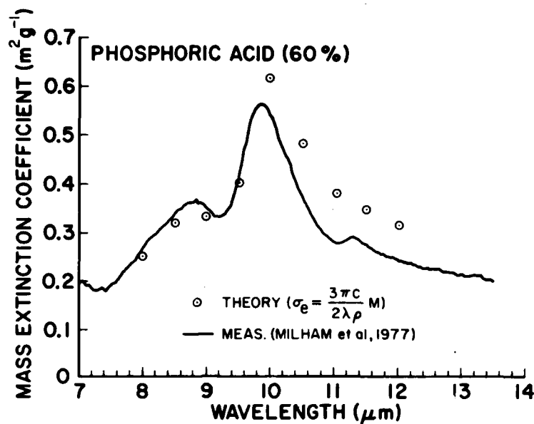
Figure 5. Same as figure 4 except for the 8\mu m \leq \lambda \leq 12\mu m spectral region.
