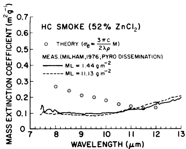
Figure 8. Same as figure 7 except for the 8\mu\text{m} \leq \lambda \leq 12\mu\text{m} spectral region. In this case, measurements are shown for two different aerosol mass loadings (M is the aerosol mass content and L the transmission chamber path length).
