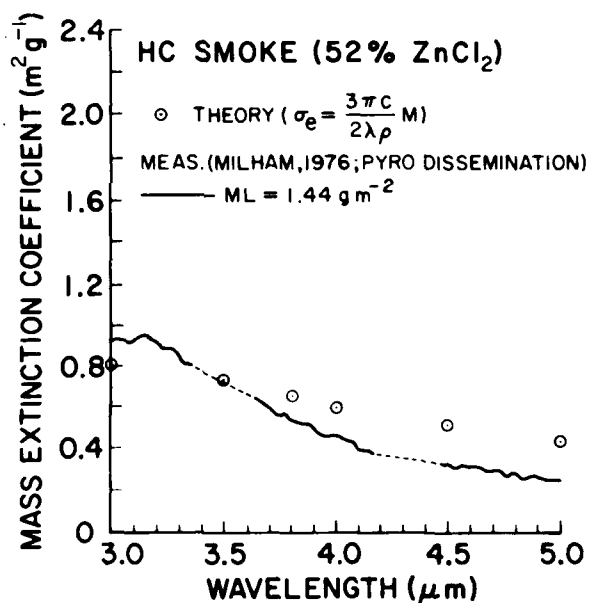
Figure 7. Values of the ratio of aerosol extinction coefficient to aerosol mass content ( \sigma_e/M in \text{m}^2\text{g}^{-1} ) predicted according to the size-distribution-independent relation (3) (open circles), and measured by Milham 1,5 (smooth curve) for HC smoke.
