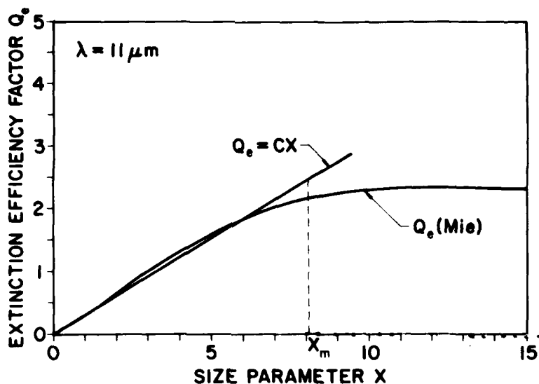
Figure 1. The efficiency factor for extinction Q_e for water droplets versus size parameter x at a wavelength \lambda = 11 \mu\text{m} (index of refraction m = 1.153 - 0.0968i ). The efficiency factor can be approximated by a straight line Q_e = cx providing x \leq x_m . The approximation overestimates the exact value of Q_e for some size parameters, but underestimates it for others (still with x \leq x_m ). These two errors tend to cancel, leading to the extinction coefficient being linearly related to the liquid water content of fogs according to equation (3).
