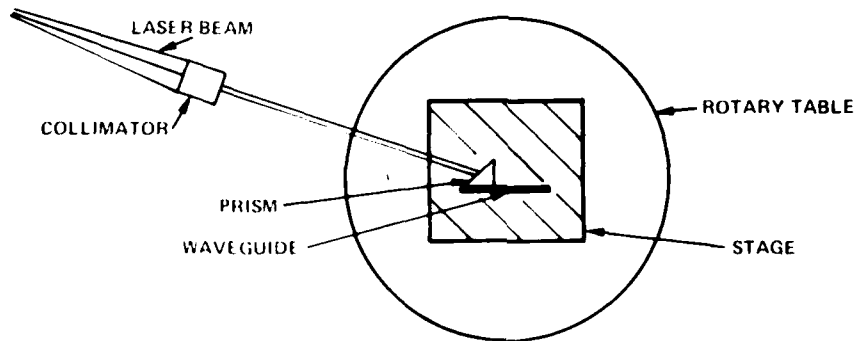
Figure 3. Experimental Facility
