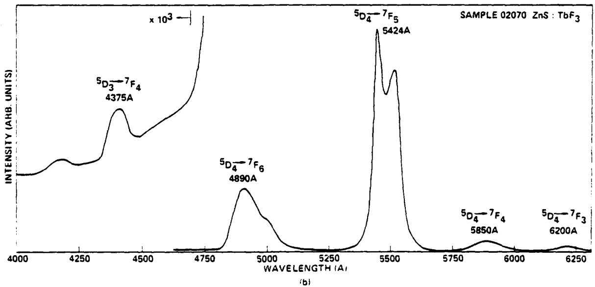
Fig. 2 Room temperature thin film electroluminescence spectrum (a) ZnS:Tb; (b) ZnS:TbF 3 .
