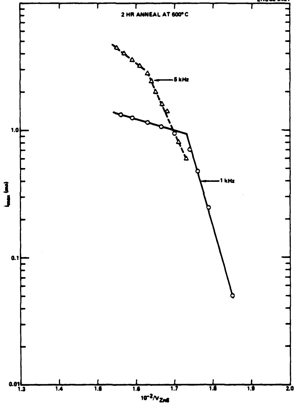
Fig. 5 Electronic current vs (\text{field across ZnS})^{-1} for ZnS:TbF 3 thin film.
