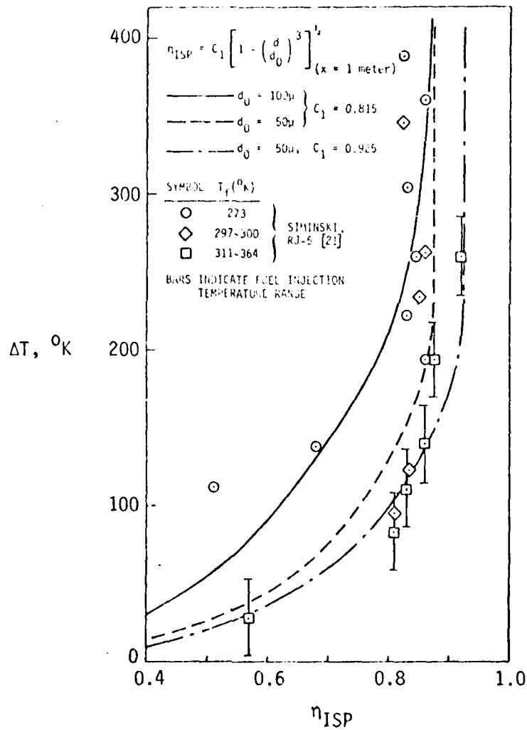
Figure 16. CORRELATION BETWEEN VAPORIZATION RATE AND ISP EFFICIENCY, RJ-5 FUEL
