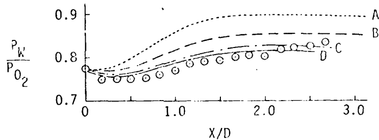
Figure 13. COMPARISON OF PREDICTED WALL STATIC PRESSURE DISTRIBUTIONS WITH COLD FLOW SUDDEN-EXPANSION COMBUSTOR DATA [18]
