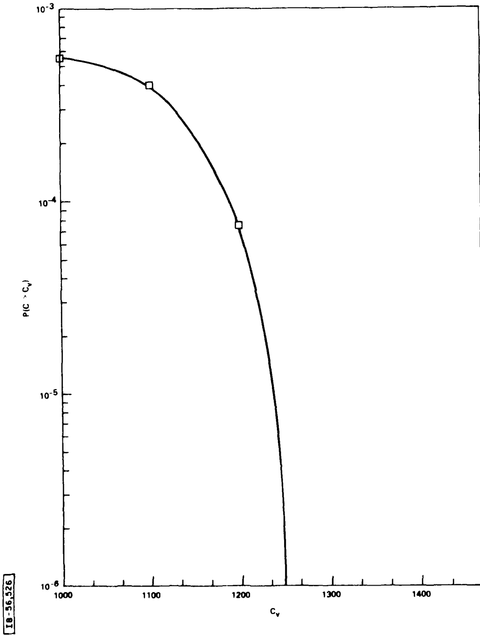
Figure 15. THE PROBABILITY DISTRIBUTION THAT THE NUMBER OF COMPUTATIONS PERFORMED FOR ERASUREFREE DECODING C IS LARGER THAN SOME NUMBER C_v (1000 \leq C_v \leq 1400) FOR (2, 1) 8 MSA
