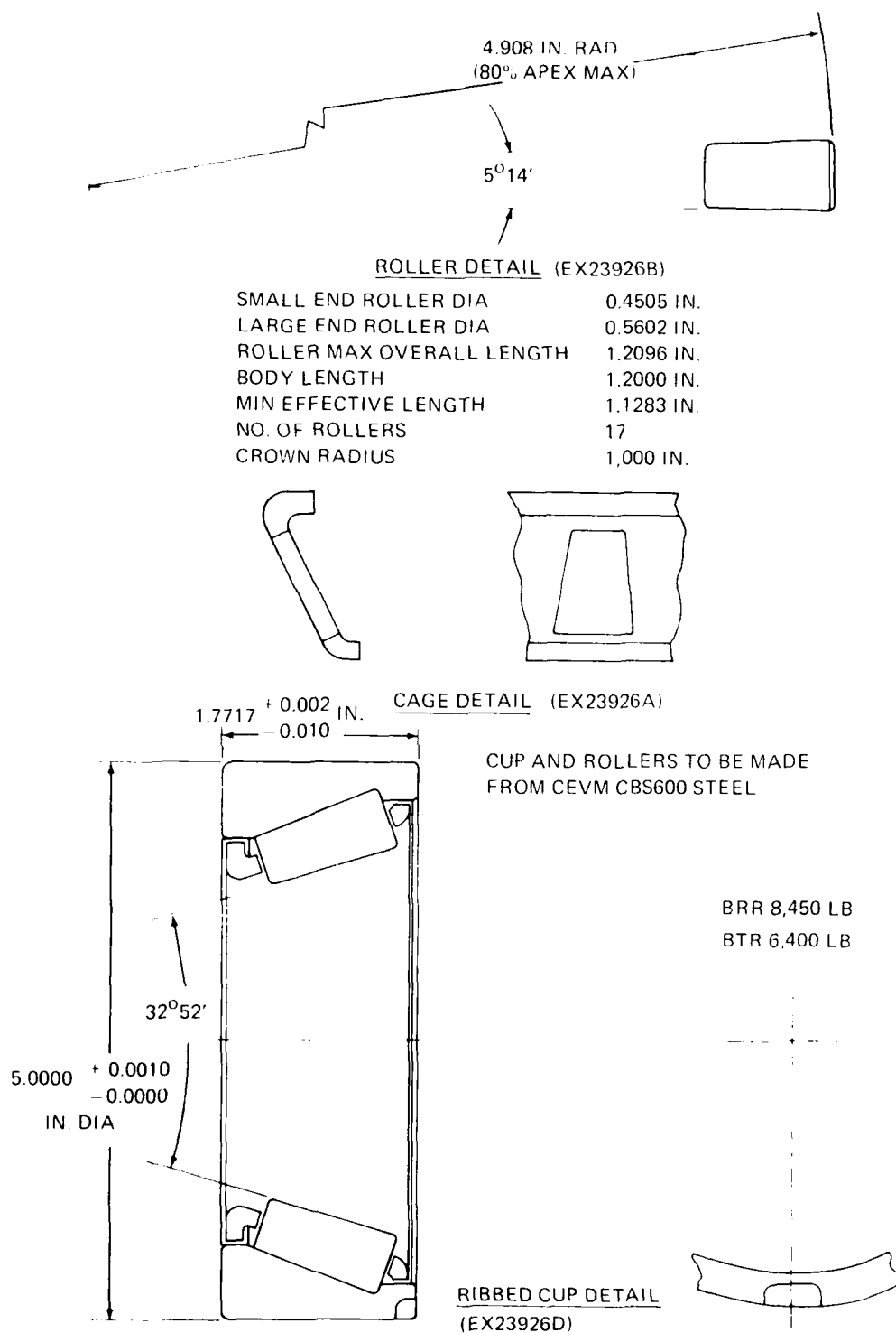
Figure 41. Design of Tapered-Roller Bearing for Test Series.
