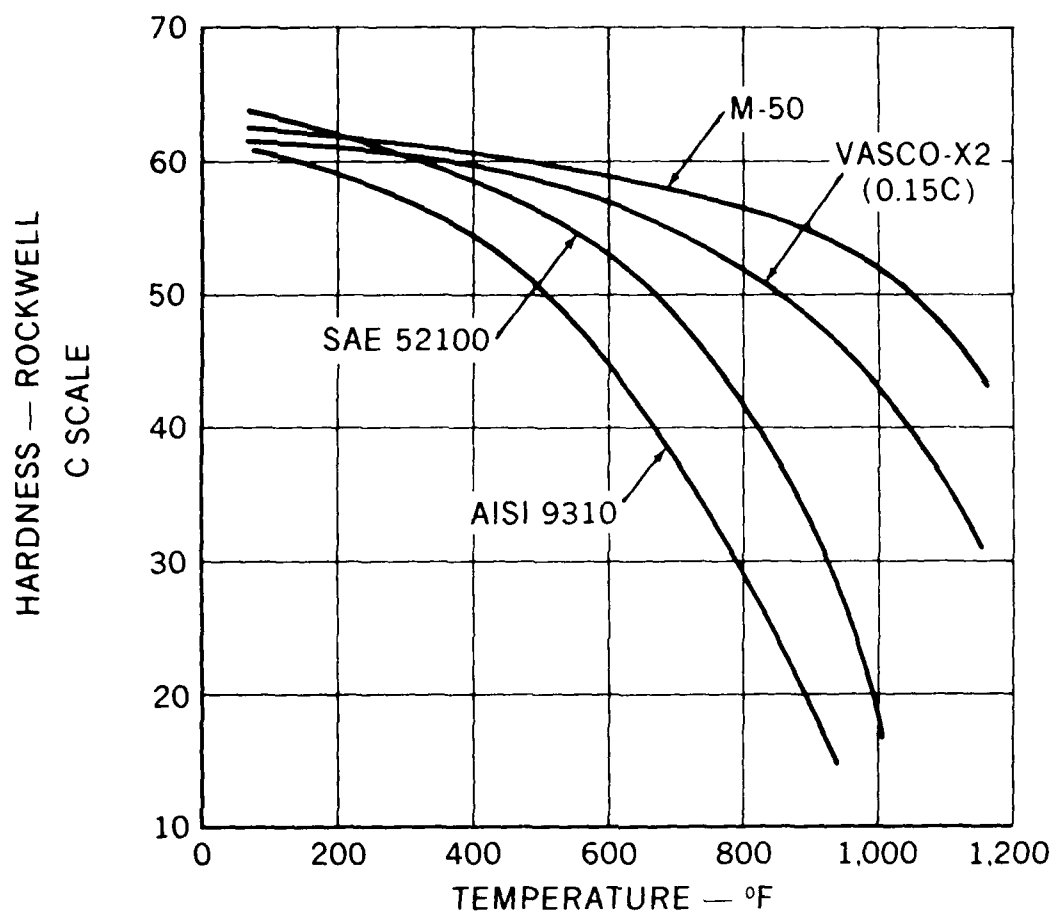
Figure 2. Hot Hardness Characteristics of Common Bearing Steels.
