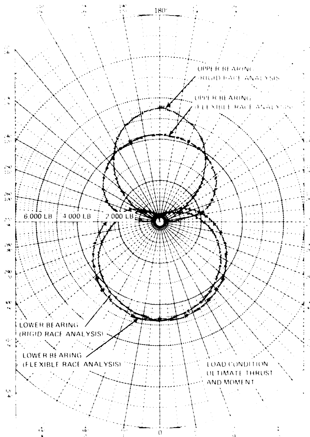
Figure 94 Rotor Shaft Support Bearing Internal Load Distribution
