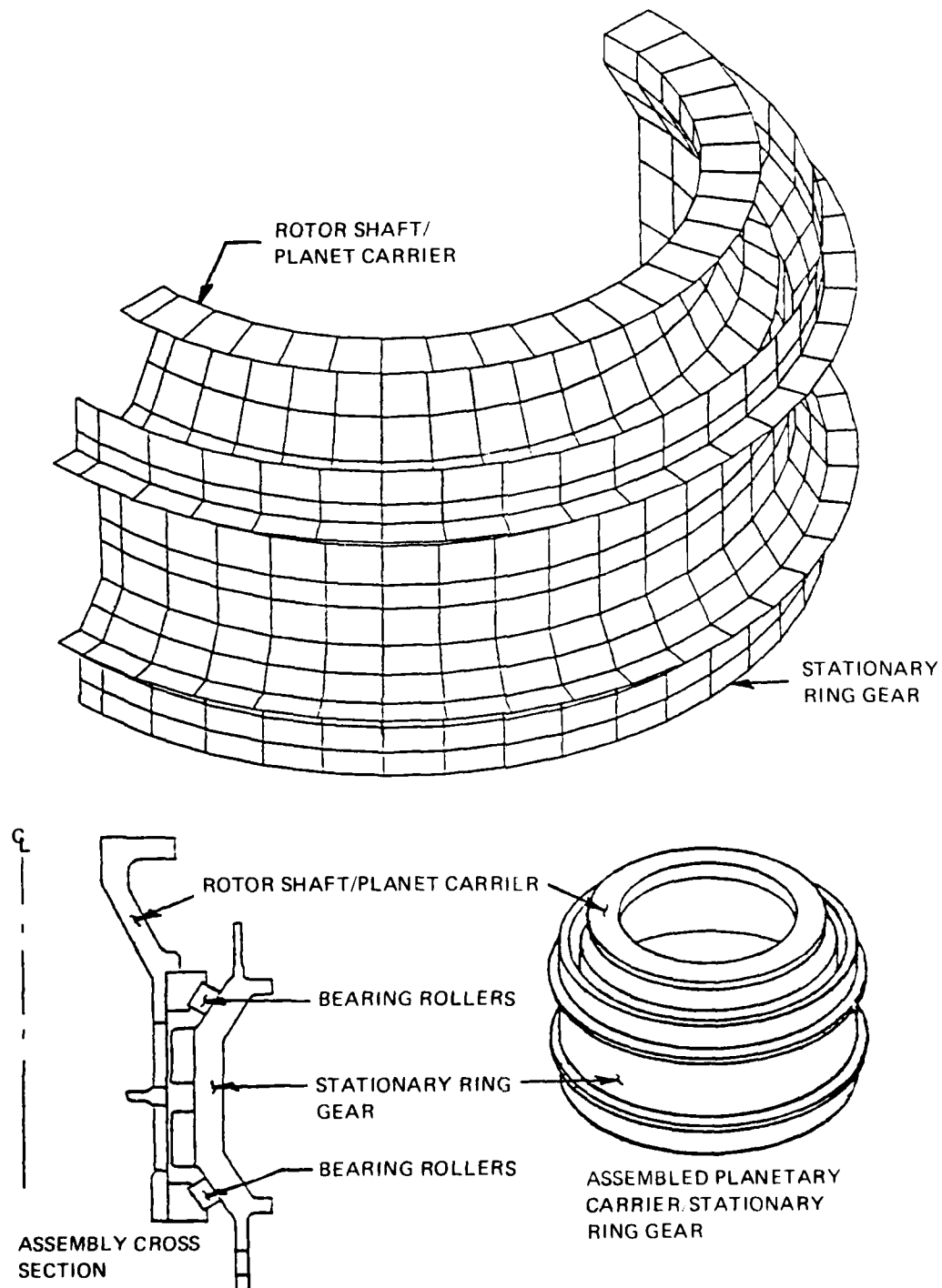
Figure 90. Finite-Element Model of a Planetary Carrier/Stationary Ring Gear.
