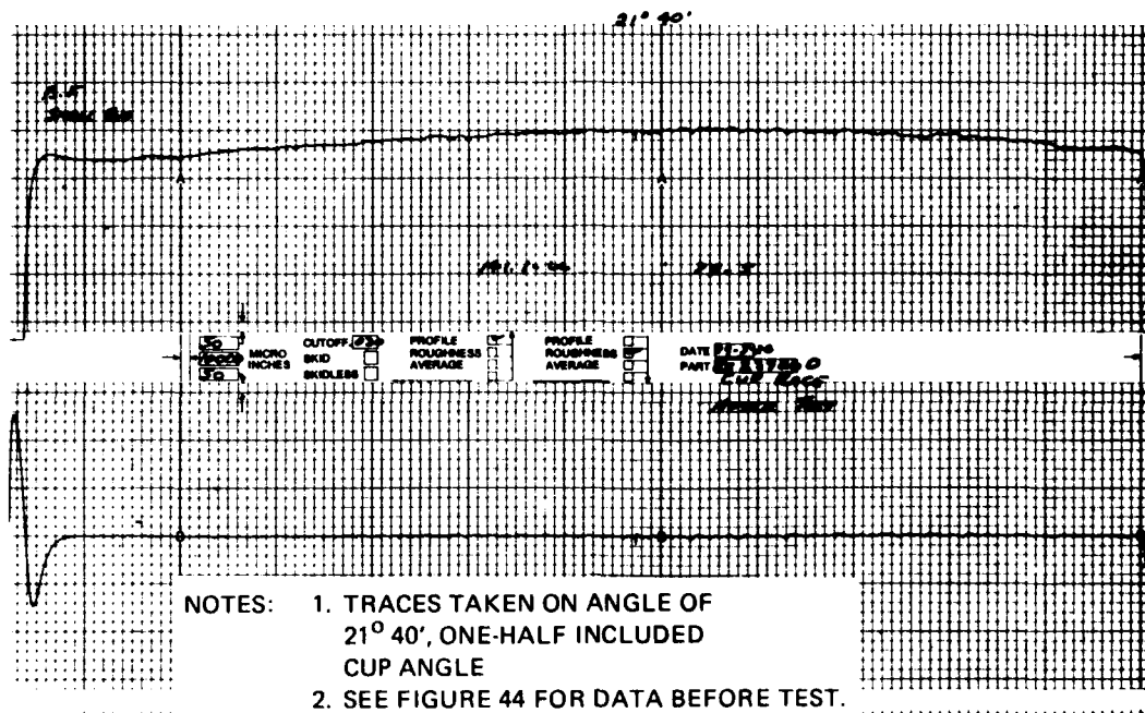
Figure 65. Profile Trace of Drive-End Cup Race After Test Setup No. 5.
