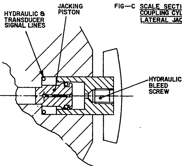
Figure 36. Description of the coupling cylinder mechanism
