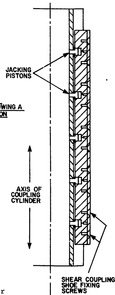
FIG-B REDUCED SCALE SECTION OF THE COUPLING CYLINDER SHOWING DISTRIBUTION OF JACKING PISTONS
