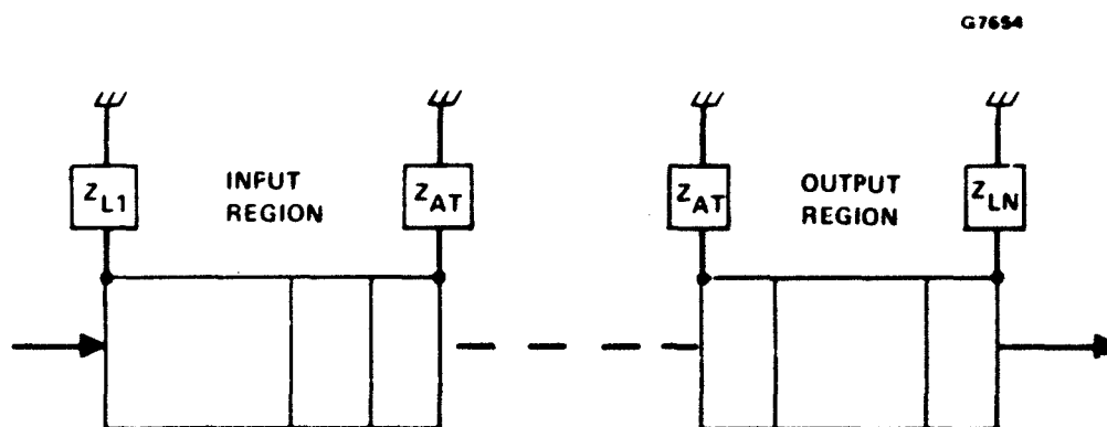
Figure 5-4 Sketch showing the TWT separated into two regions, with the attenuator load Z_{AT} serving as output load for the first region and input load for the second region.
