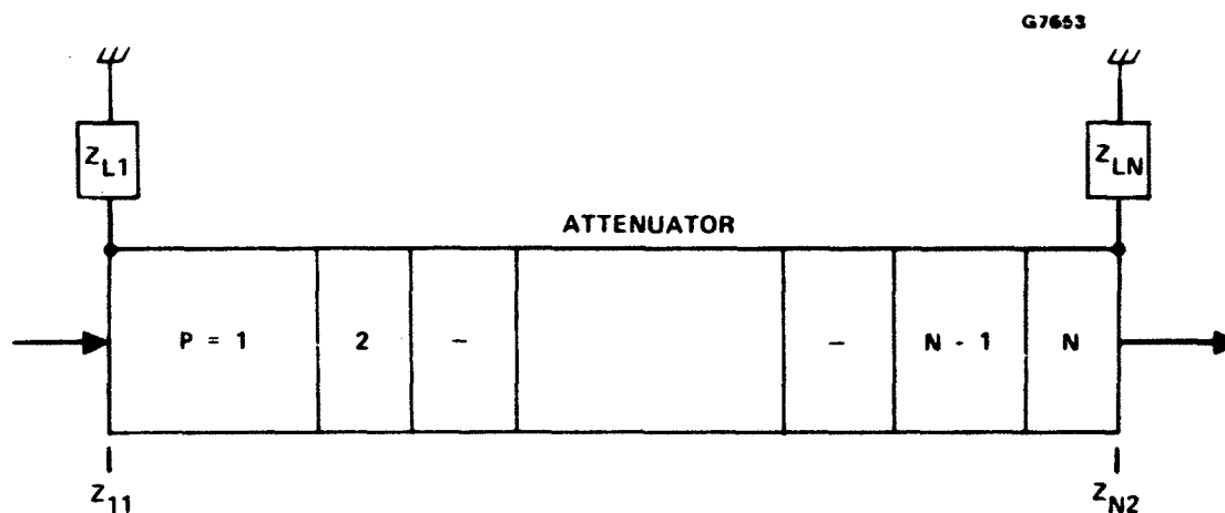
Figure 5-3 Schematic diagram of a sectioned TWT with arbitrary input and output loads Z_{L1} and Z_{LN} .
