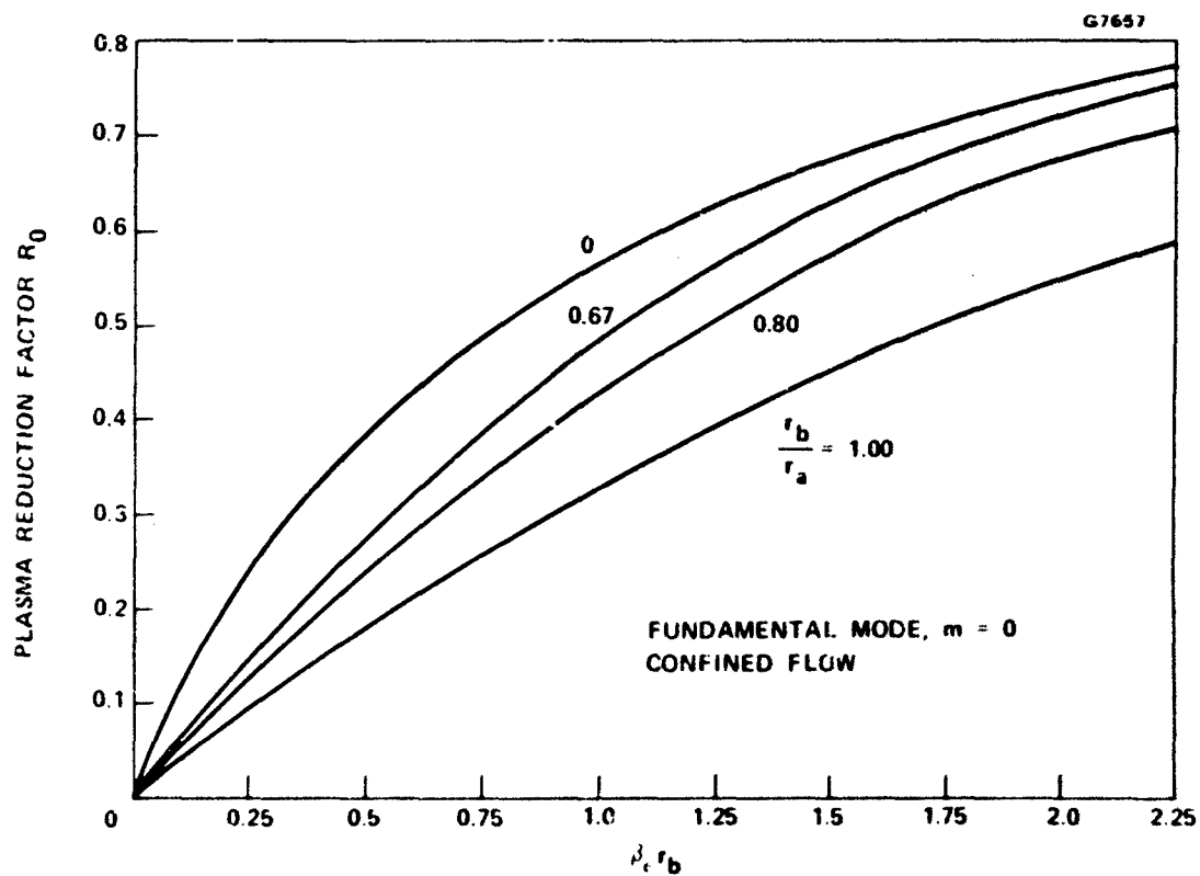
Figure 6-2 Plasma frequency reduction factor R_0 for forward wave interaction and confined flow.
