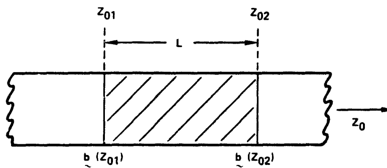
Figure 4-6 Schematic illustration of one uniform helix section.
