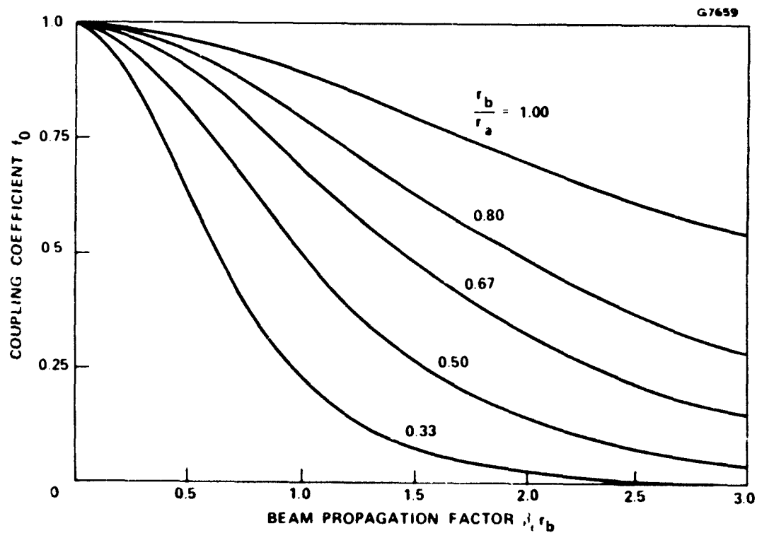
Figure 6-4 Beam-circuit coupling coefficient f_0 for forward wave interaction ( m = 0 ) and confined flow.
