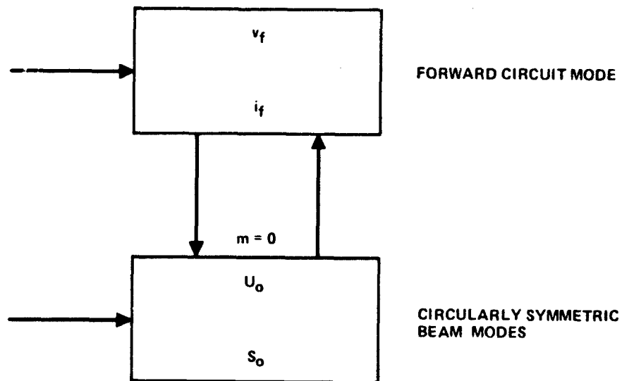
Figure 4-4 Schematic diagram of forward interaction, and the rf variables involved.
