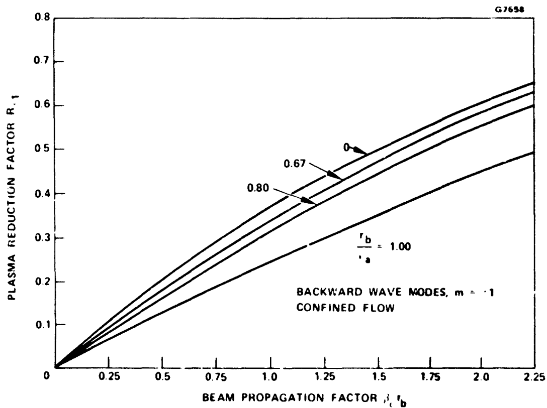
Figure 6-3 Plasma frequency reduction factor R_1 for backward wave interaction and confined flow.
