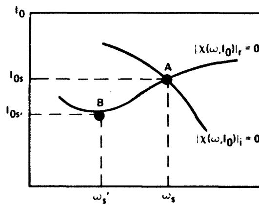
Figure 5-1 Illustration of instability diagram for backward wave oscillations.
