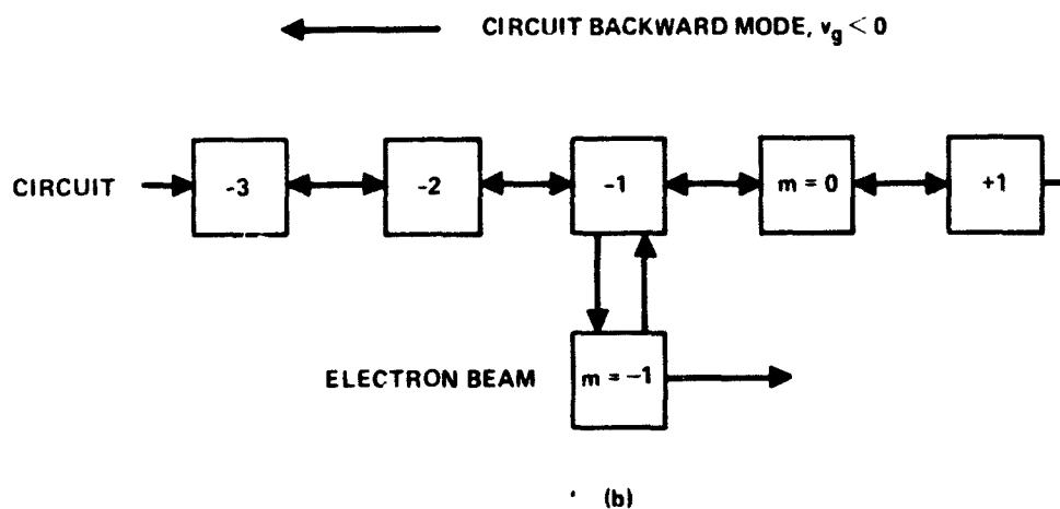
Figure 4-3 Schematic diagram illustrating the circuit and beam harmonics involved in: a) forward interaction, b) backward interaction in a left-handed helix.
