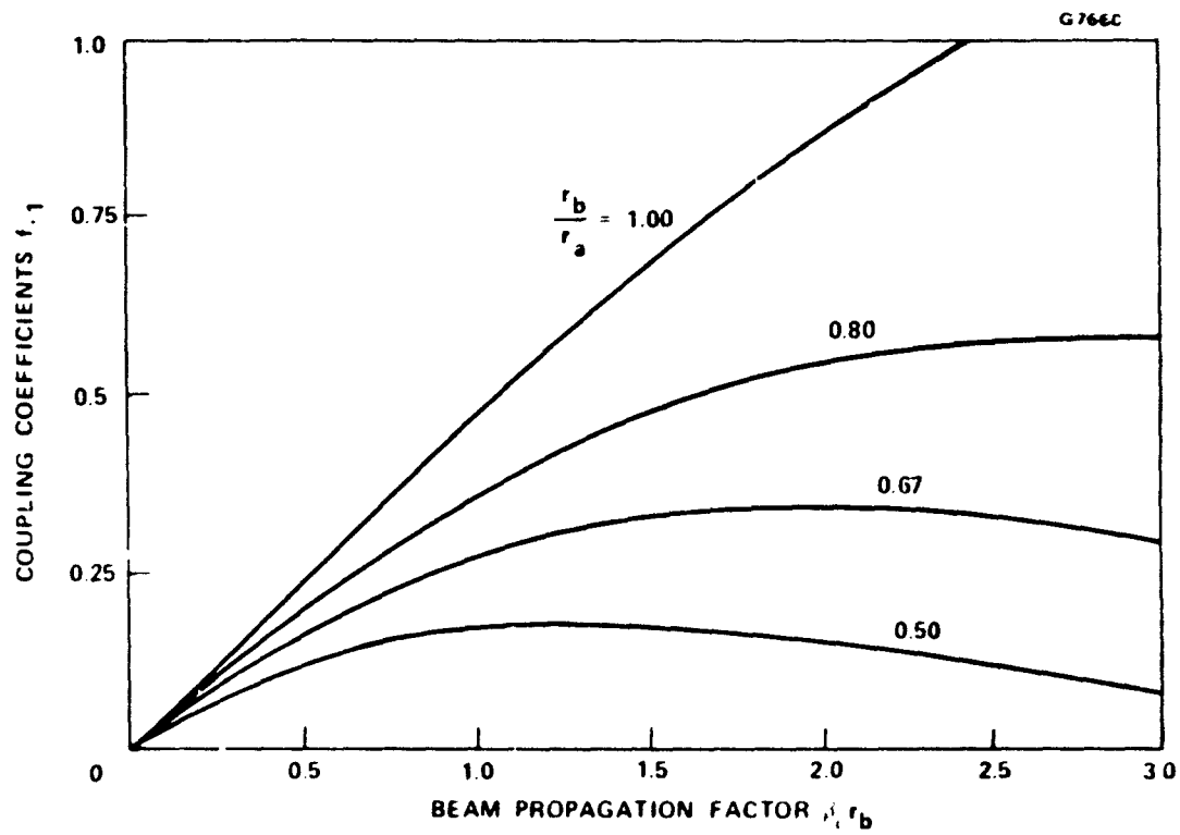
Figure 6-5 Beam-circuit coupling coefficient f_{+1} for backward wave interaction ( m = \pm 1 ) and confined flow.
