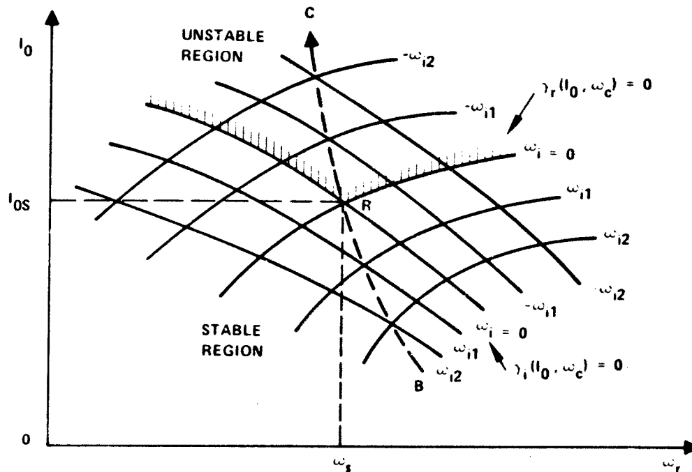
Figure 5-2 Sketch illustrating the nature of backward wave instabilities. The region above the shaded outline is unstable.
