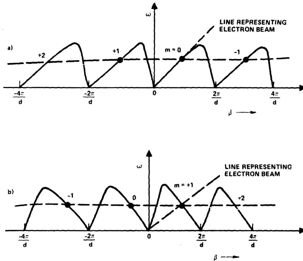
Figure 4-2 Dispersion diagram of right-handed helix. a) Forward wave interaction in the m = 0 mode b) Backward wave interaction in the m = +1 mode
