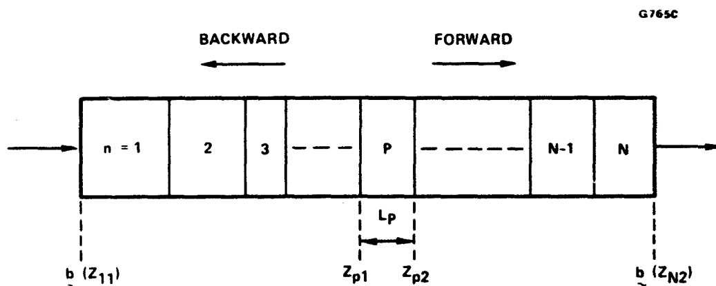
Figure 4-7 Schematic configuration of a multisection TWT consisting of a total of n uniform, but different sections.
