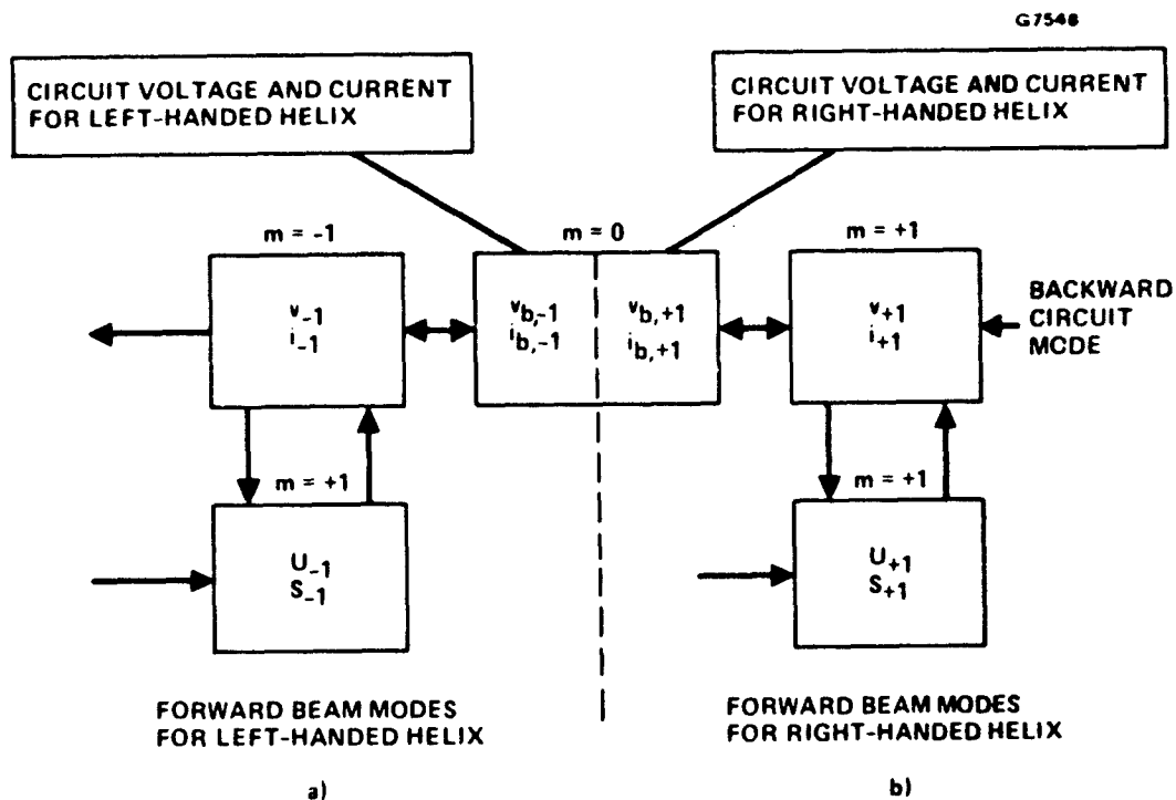
Figure 4-5 Schematic diagram of backward interaction, and the rf variables involved: a) left-handed helix, b) right-handed helix.
