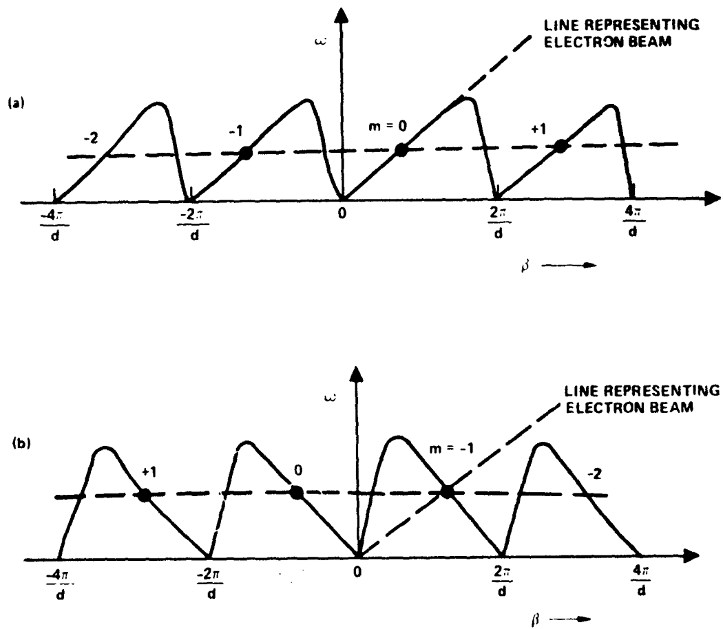
Figure 4-1 Dispersion diagram of left-handed helix. a) Forward wave interaction in the m = 0 mode b) Backward wave interaction in the m = -1 mode
