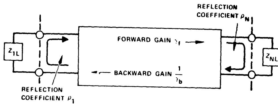
Figure 5-5 Schematic illustration of the condition (5.36) of unit; loop gain as criterion for backward wave oscillations.
