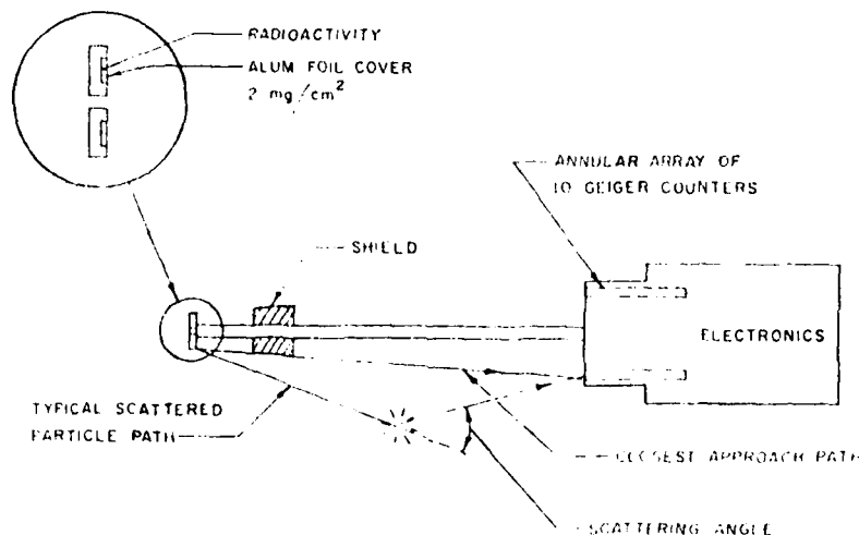
Figure 1.1 Cross Section of Original Betasonde Showing Density Measurement Concept
