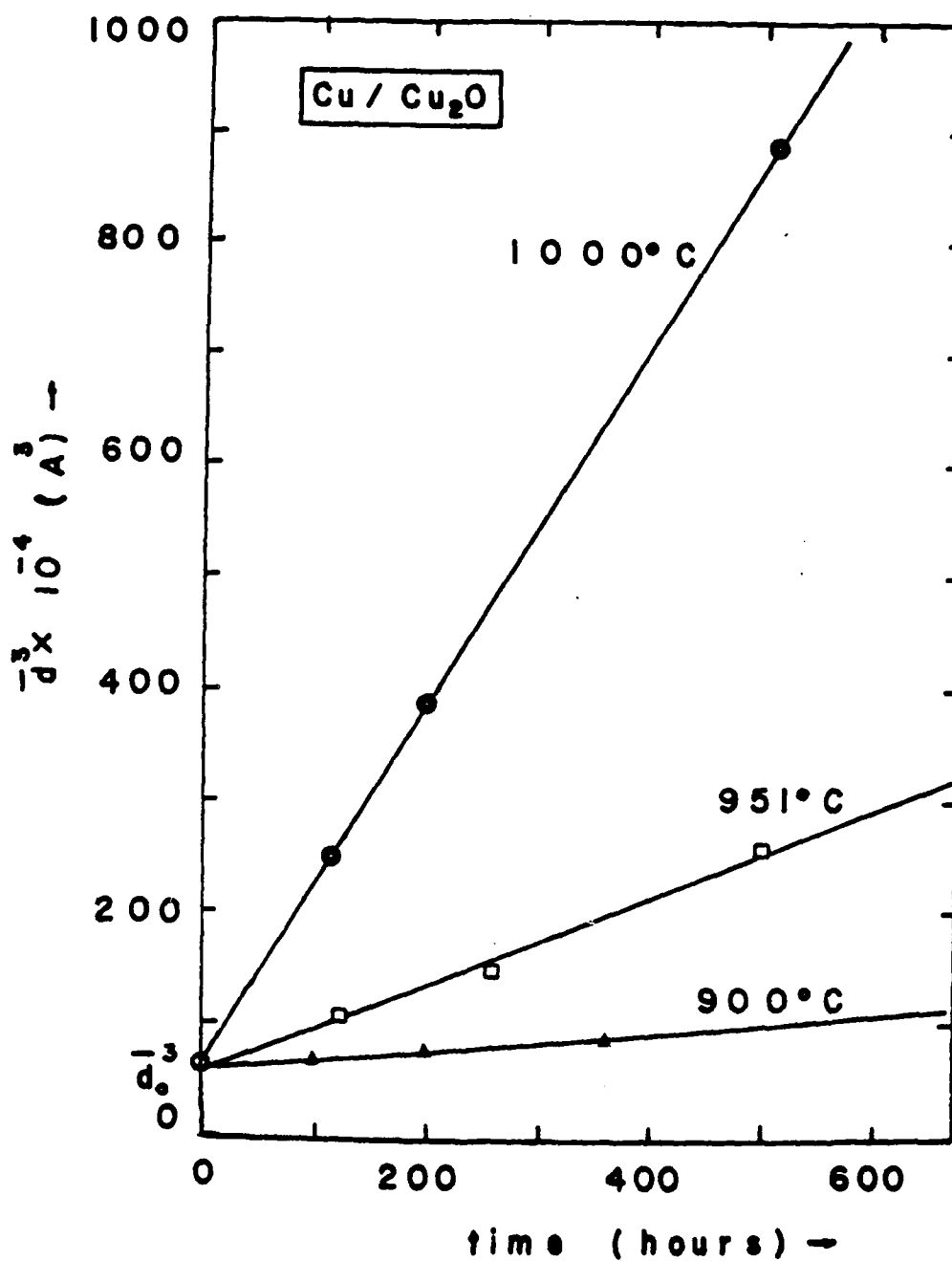
Figure 16. Variation of average particle size cubed as a function of time for \text{TiO}_2 oxide particles coarsened in \text{Cu/Cu}_2\text{O} .
