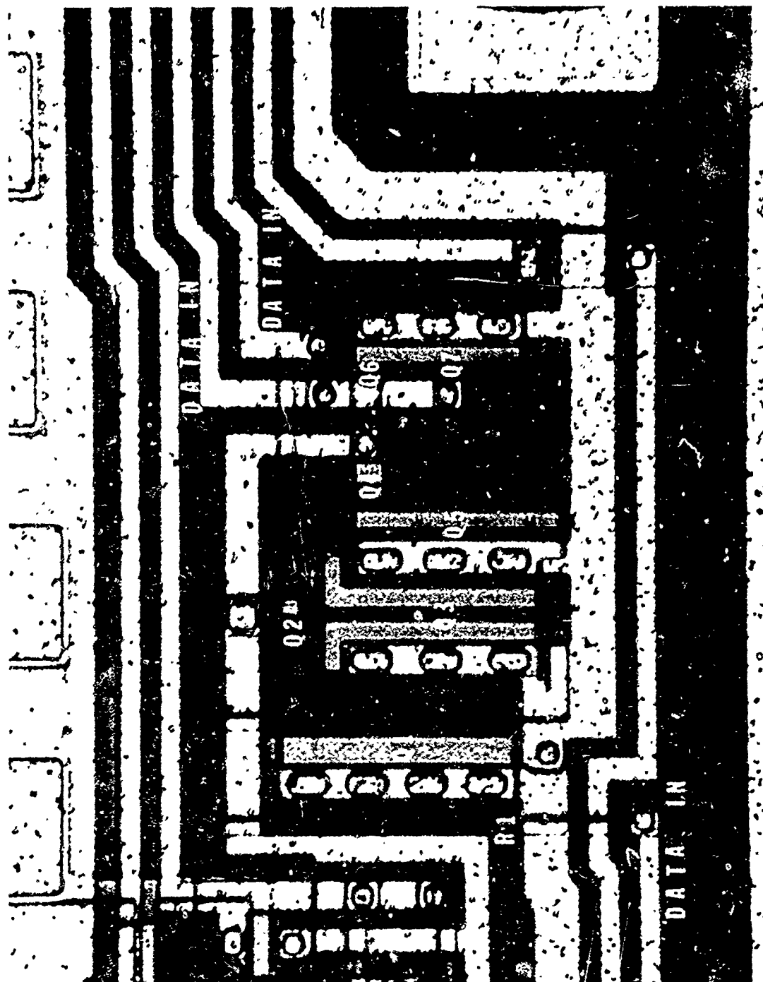
Photo 5-14 Light Photograph of the Data IN Buffer. Mag. - 460X
