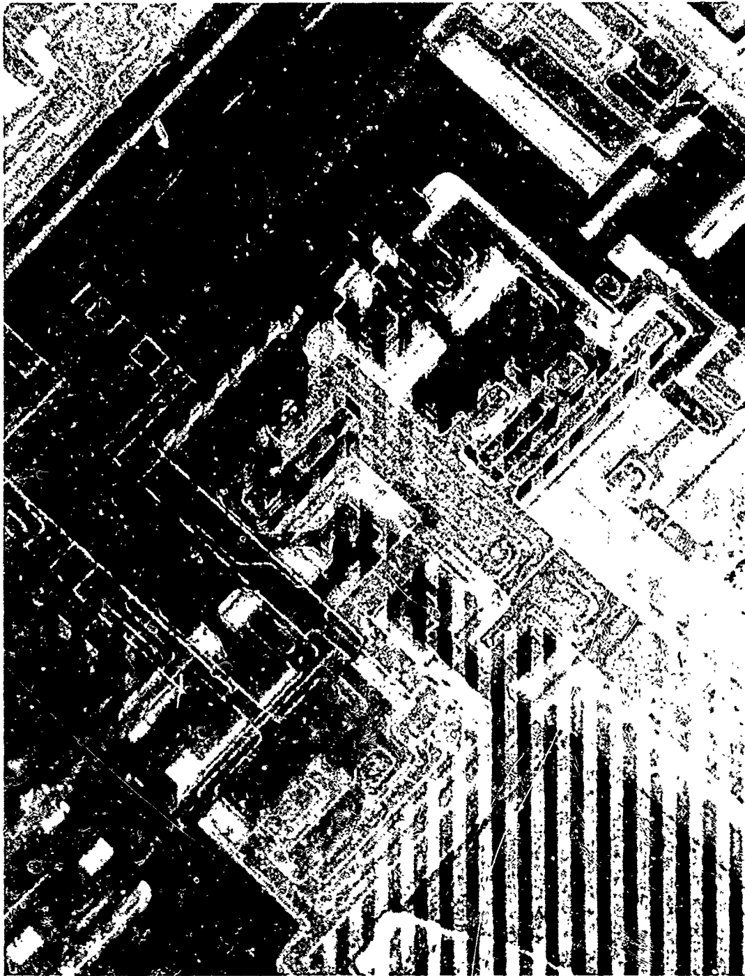
Photo 6 Voltage Contrast Micrograph Showing Beam Blanked Functional Mapping at 40 KHz. 5 KV, Mag. - 500X
