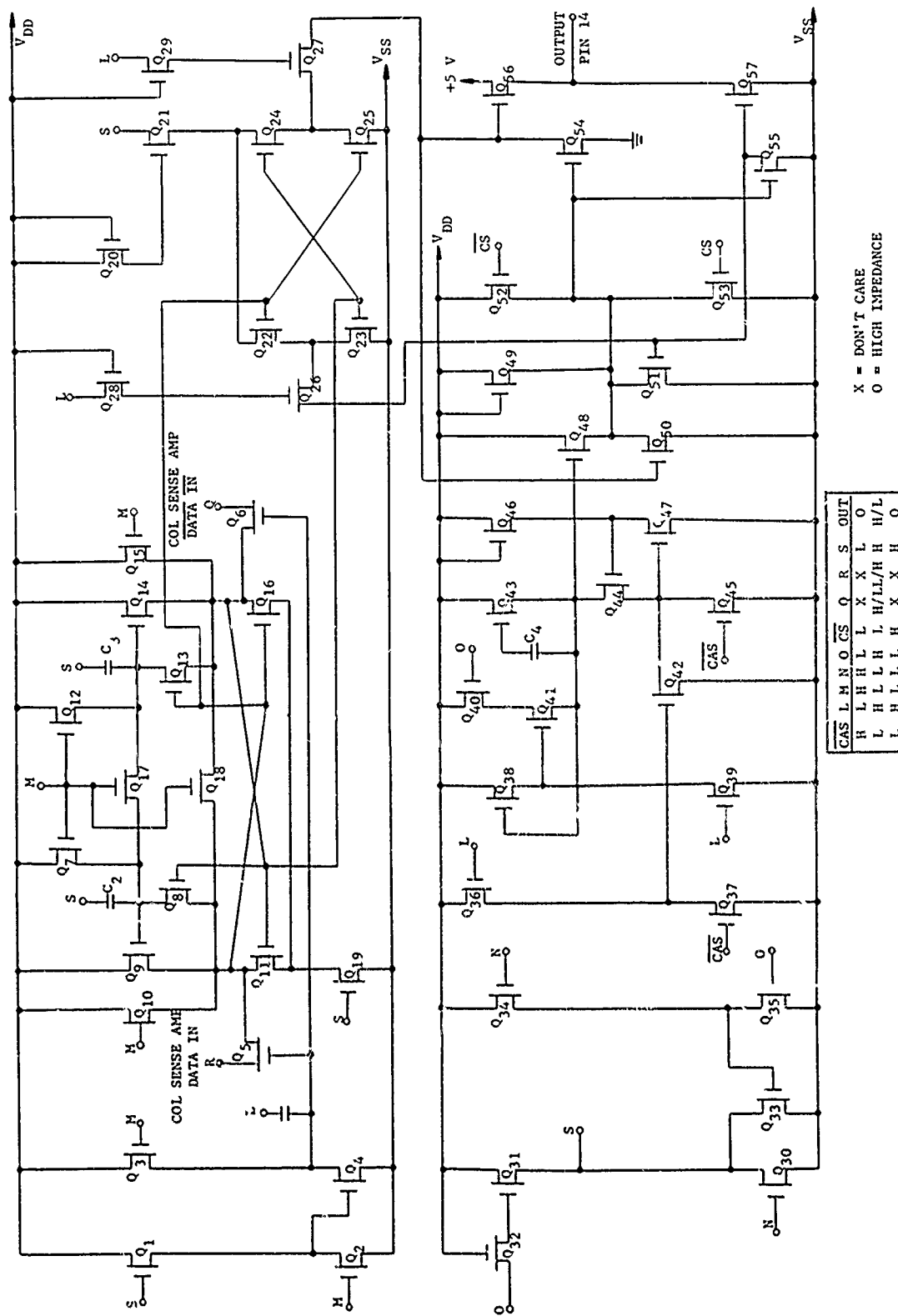
Figure 6-28 Schematic, Data Output
