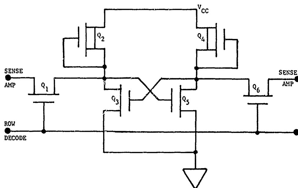
Figure 5-17 Schematic, Memory Cell
