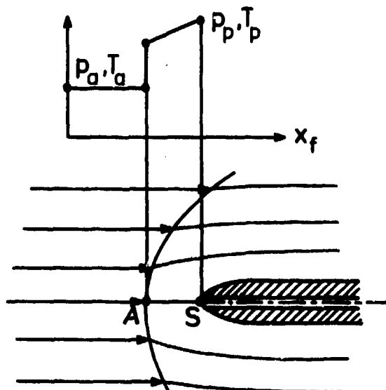
Fig.3 Probe tip in supersonic flow with detached shock wave. S stagnation point, A vertex of shock wave.
