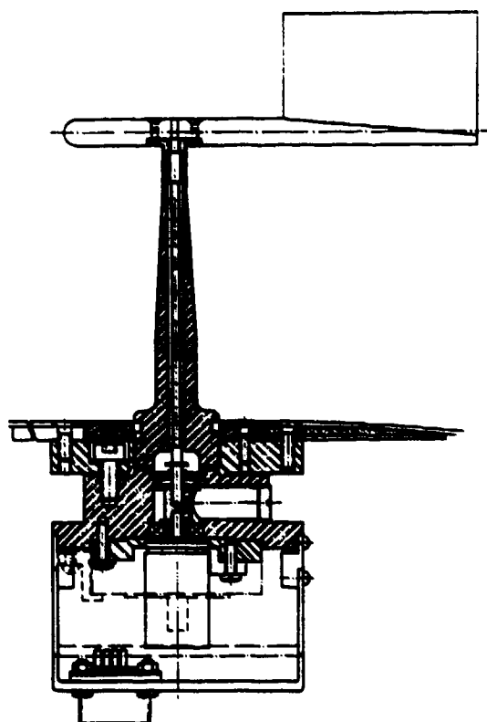
Fig.77 Vane-type flow-direction-indicator with synchro-pick-up for flight tests [119].
