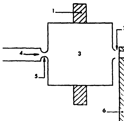
Fig.110 Working principle of modulated ejector for the dynamic pressure calibration. 1) pressure pick-up, 2) exit nozzle, 3) cavity, 4) compressed gas inlet, 5) inlet nozzle, 6) modulation disk. ONERA, France.
