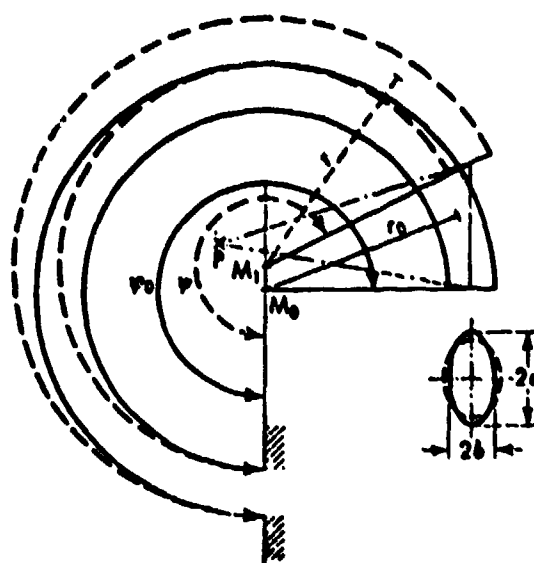
Fig.79 Principle of operation of a Bourdon tube.
