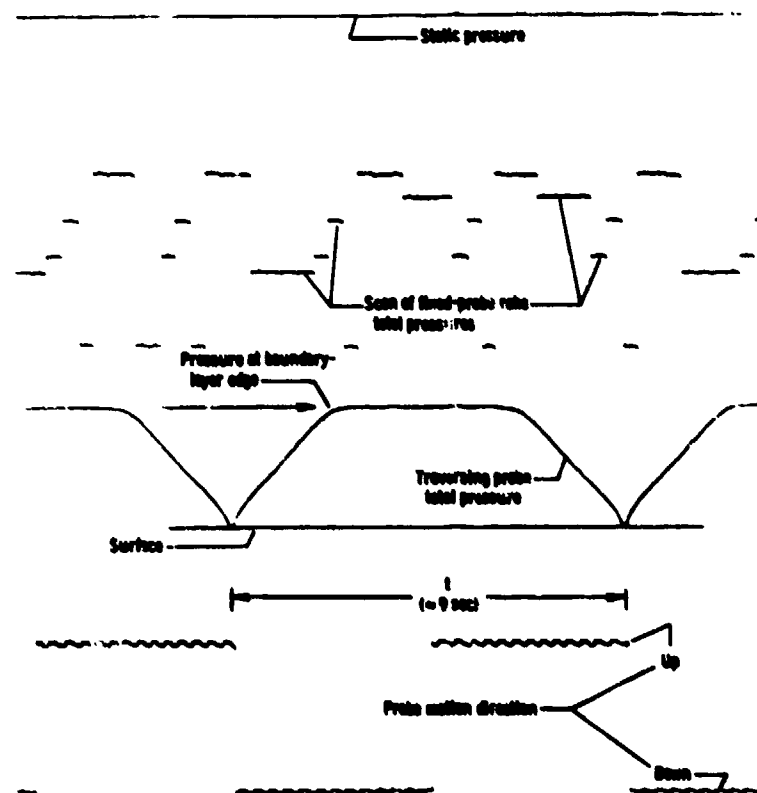
Fig.144 Analog read-out from the F-104 installation of fig.143.
