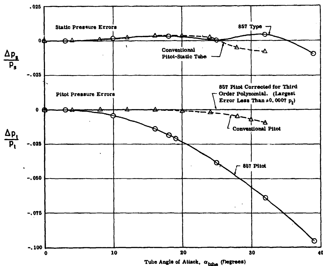
Fig.71 Comparison of typical pitot and static pressure errors for conventional and blunt tip pitot-static tubes (Rosemount model 857, M = 0.4 ).
