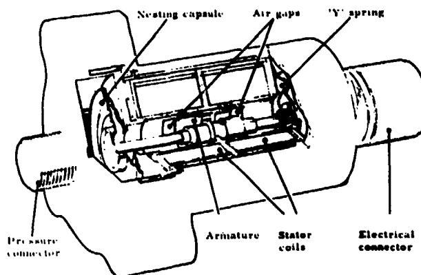
Fig.83 Inductor pressure transmitter (Smith Industries Ltd U.K.)
