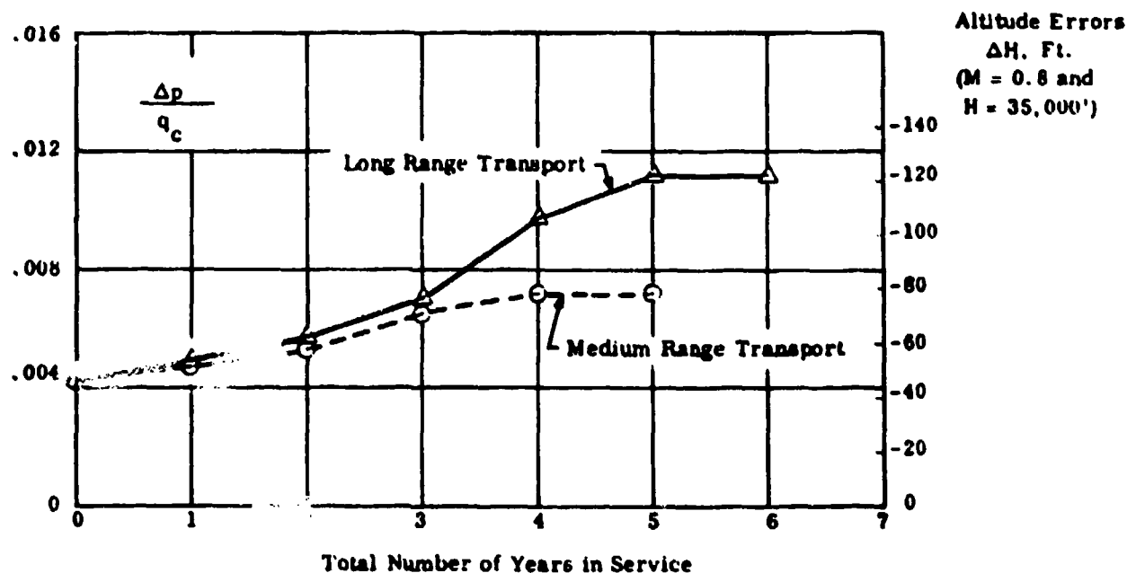
Fig.53 Predicted variation with time of static source errors for aerodynamically compensated Pitot-static tubes of typical wide body transport aircraft.
