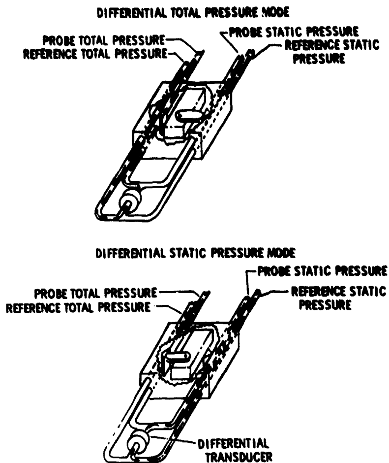
Fig.149 Pressure transducer switching valve for the arrangement of fig.148.
