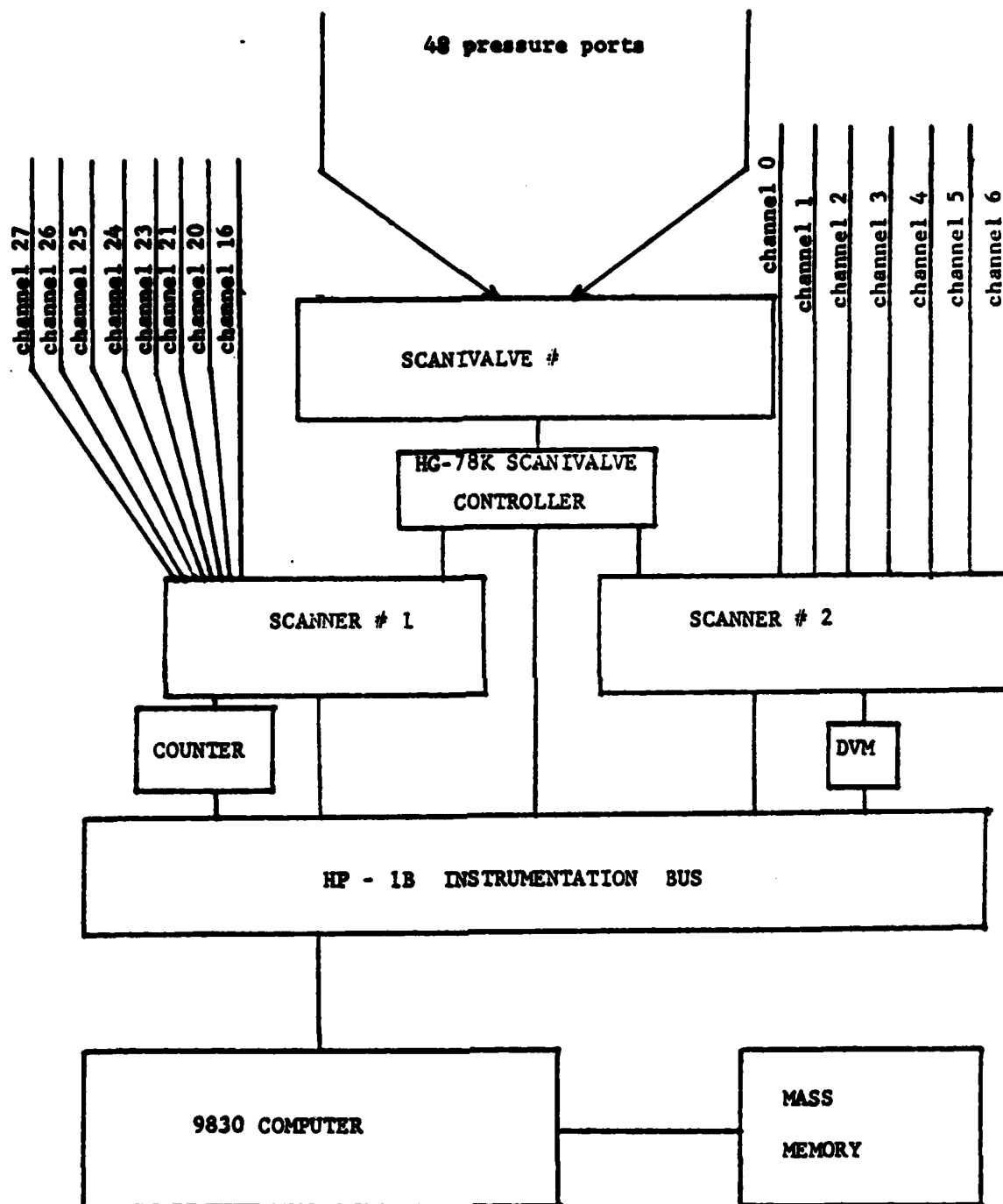
FIGURE 6. Instrumentation System
