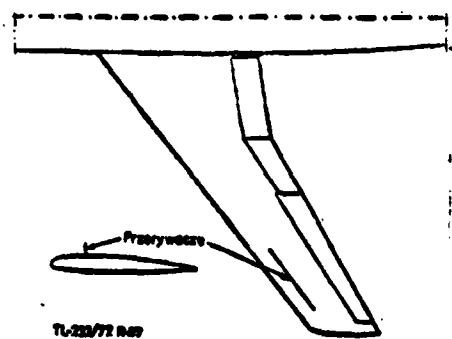
Fig. 27 Spoiler placement
